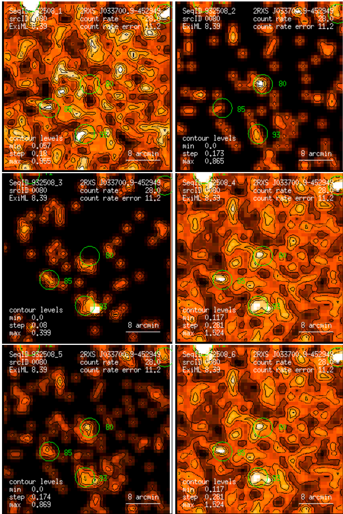
Figure 80: RASS 932508: detection 0080: band rate images, Gaussian filter: (1) PSPC channels 11 – 41, (2) 52 – 90, (3) 91 – 201, (4) 11 – 235, (5) 52 – 201, (6) 11 – 201. Broad band rates in counts/ks. Band rate contour levels in counts/ks/arcmin 2 .
