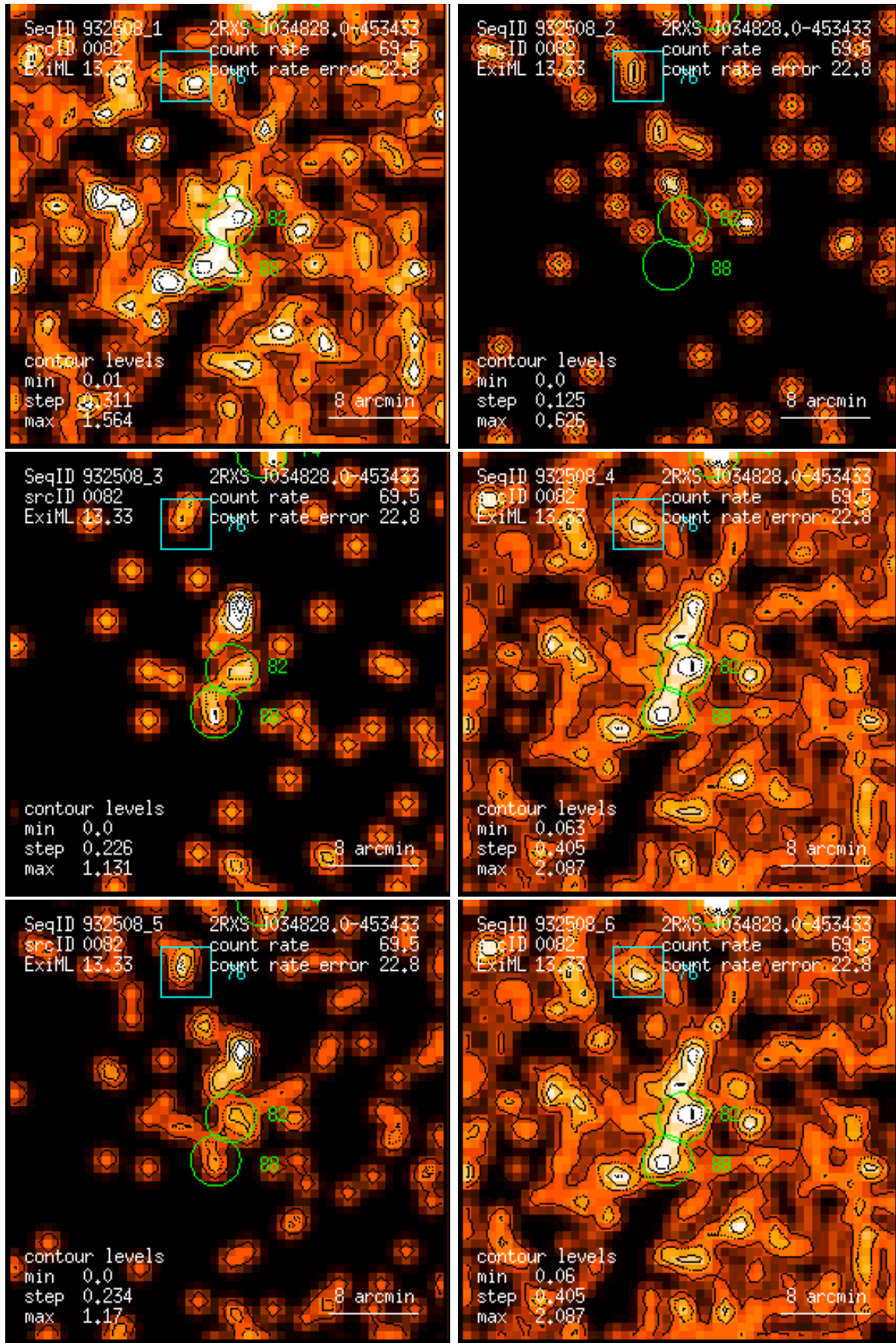
Figure 82: RASS 932508: detection 0082: band rate images, Gaussian filter: (1) PSPC channels 11 – 41, (2) 52 – 90, (3) 91 – 201, (4) 11 – 235, (5) 52 – 201, (6) 11 – 201. Broad band rates in counts/ks. Band rate contour levels in counts/ks/arcmin 2 .
