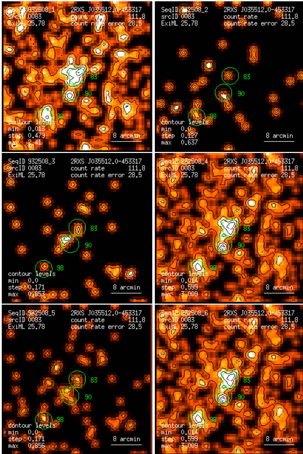
Figure 83: RASS 932508: detection 0083: band rate images, Gaussian filter: (1) PSPC channels 11 – 41, (2) 52 – 90, (3) 91 – 201, (4) 11 – 235, (5) 52 – 201, (6) 11 – 201. Broad band rates in counts/ks. Band rate contour levels in counts/ks/arcmin 2 .
