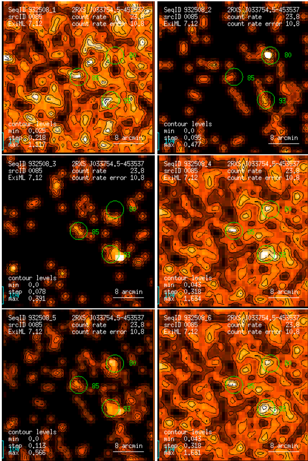
Figure 85: RASS 932508: detection 0085: band rate images, Gaussian filter: (1) PSPC channels 11 – 41, (2) 52 – 90, (3) 91 – 201, (4) 11 – 235, (5) 52 – 201, (6) 11 – 201. Broad band rates in counts/ks. Band rate contour levels in counts/ks/arcmin 2 .
