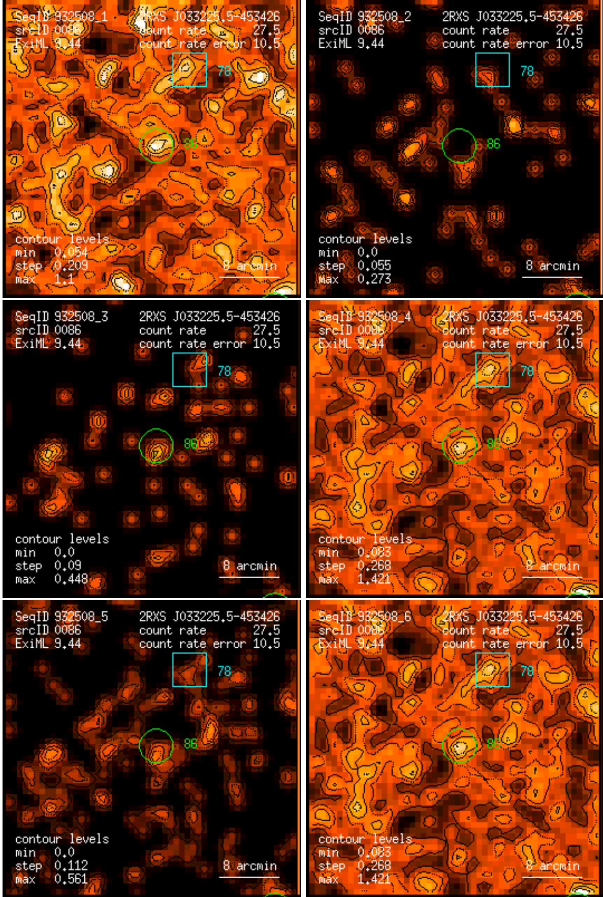
Figure 86: RASS 932508: detection 0086: band rate images, Gaussian filter: (1) PSPC channels 11 – 41, (2) 52 – 90, (3) 91 – 201, (4) 11 – 235, (5) 52 – 201, (6) 11 – 201. Broad band rates in counts/ks. Band rate contour levels in counts/ks/arcmin 2 .
