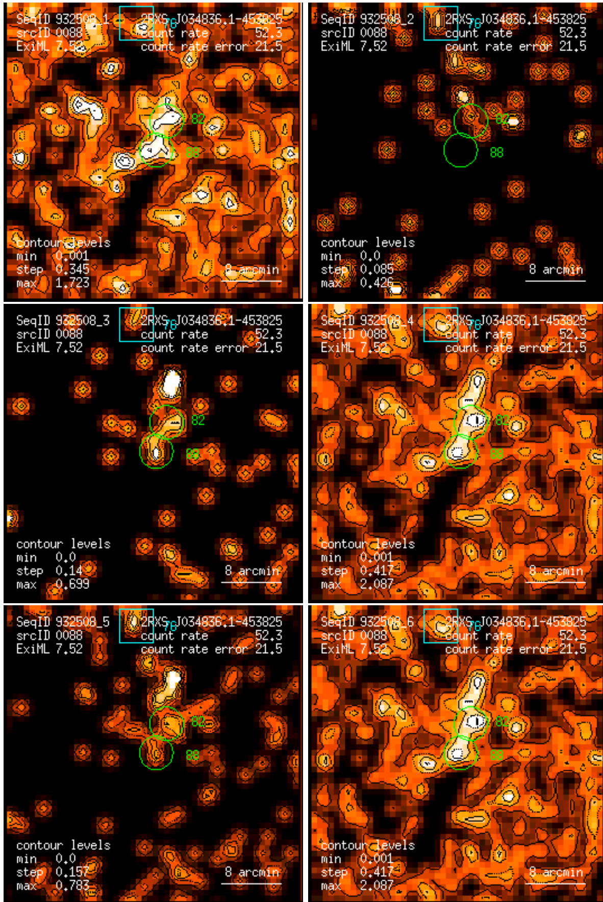
Figure 88: RASS 932508: detection 0088: band rate images, Gaussian filter: (1) PSPC channels 11 – 41, (2) 52 – 90, (3) 91 – 201, (4) 11 – 235, (5) 52 – 201, (6) 11 – 201. Broad band rates in counts/ks. Band rate contour levels in counts/ks/arcmin 2 .
