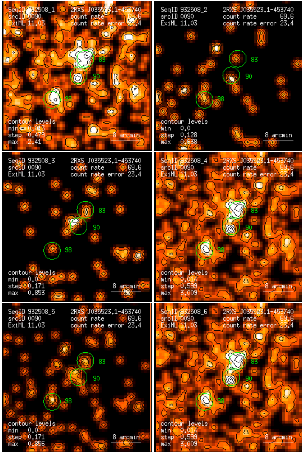
Figure 90: RASS 932508: detection 0090: band rate images, Gaussian filter: (1) PSPC channels 11 – 41, (2) 52 – 90, (3) 91 – 201, (4) 11 – 235, (5) 52 – 201, (6) 11 – 201. Broad band rates in counts/ks. Band rate contour levels in counts/ks/arcmin 2 .
