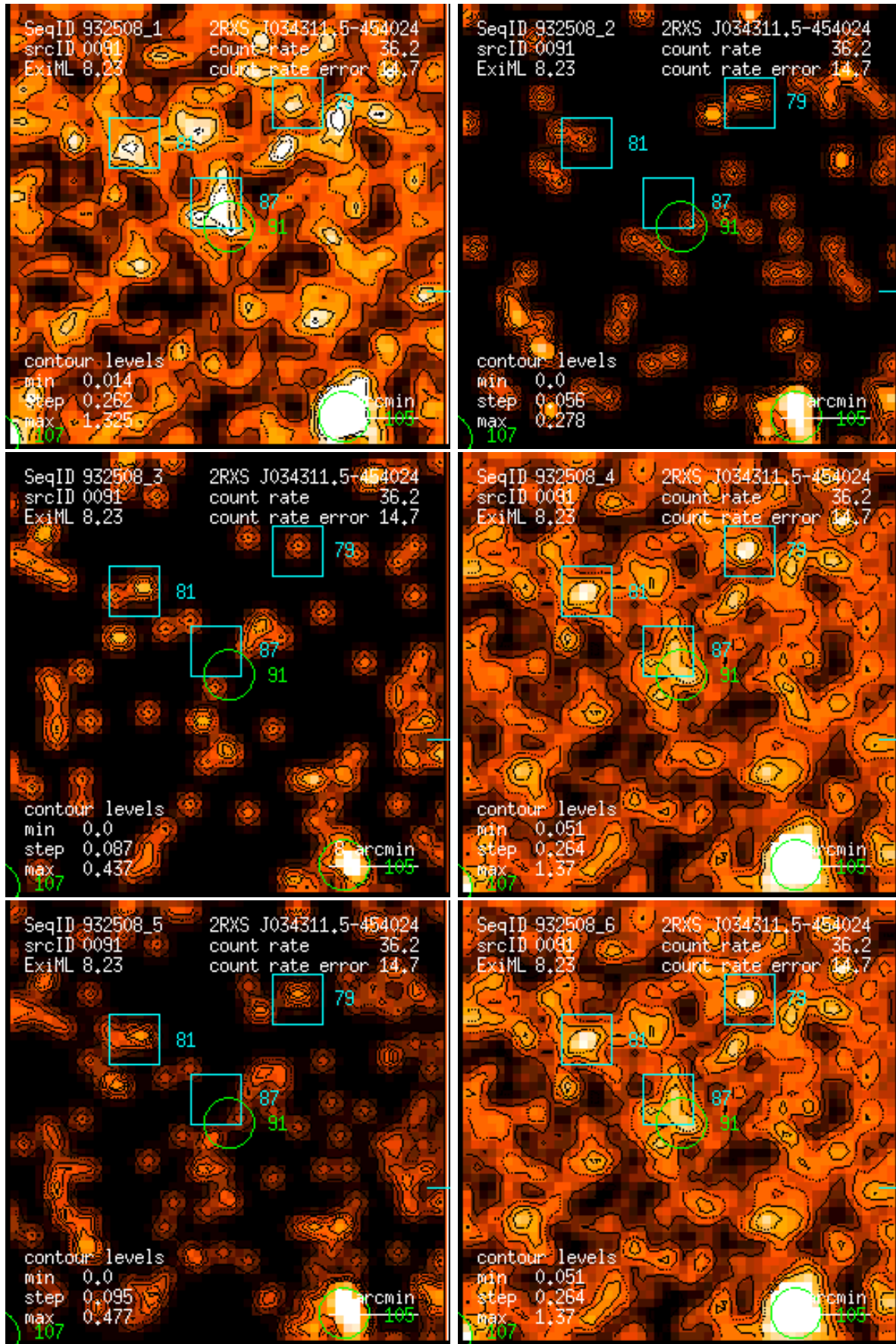
Figure 91: RASS 932508: detection 0091: band rate images, Gaussian filter: (1) PSPC channels 11 – 41, (2) 52 – 90, (3) 91 – 201, (4) 11 – 235, (5) 52 – 201, (6) 11 – 201. Broad band rates in counts/ks. Band rate contour levels in counts/ks/arcmin 2 .
