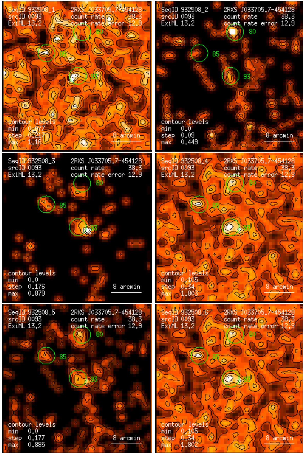
Figure 93: RASS 932508: detection 0093: band rate images, Gaussian filter: (1) PSPC channels 11 – 41, (2) 52 – 90, (3) 91 – 201, (4) 11 – 235, (5) 52 – 201, (6) 11 – 201. Broad band rates in counts/ks. Band rate contour levels in counts/ks/arcmin 2 .
