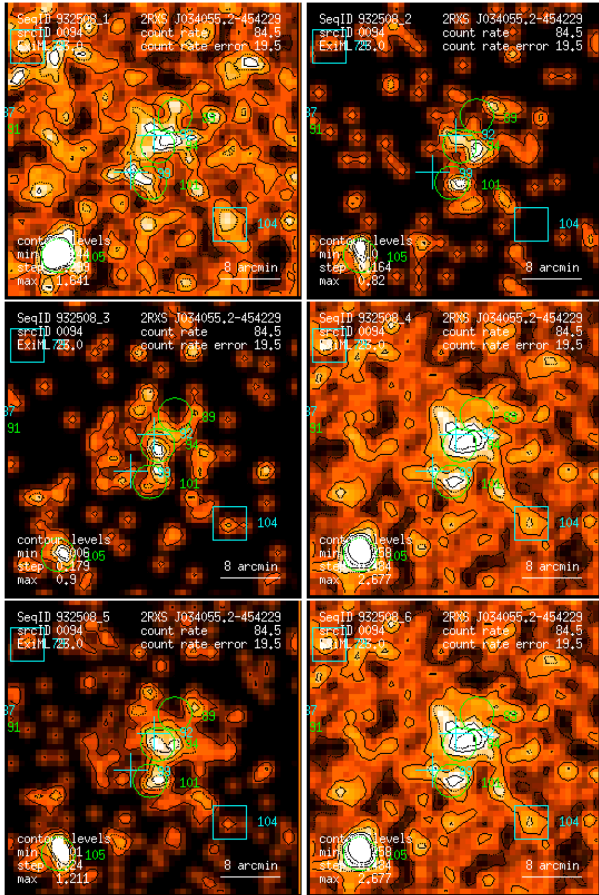
Figure 94: RASS 932508: detection 0094: band rate images, Gaussian filter: (1) PSPC channels 11 – 41, (2) 52 – 90, (3) 91 – 201, (4) 11 – 235, (5) 52 – 201, (6) 11 – 201. Broad band rates in counts/ks. Band rate contour levels in counts/ks/arcmin 2 .
