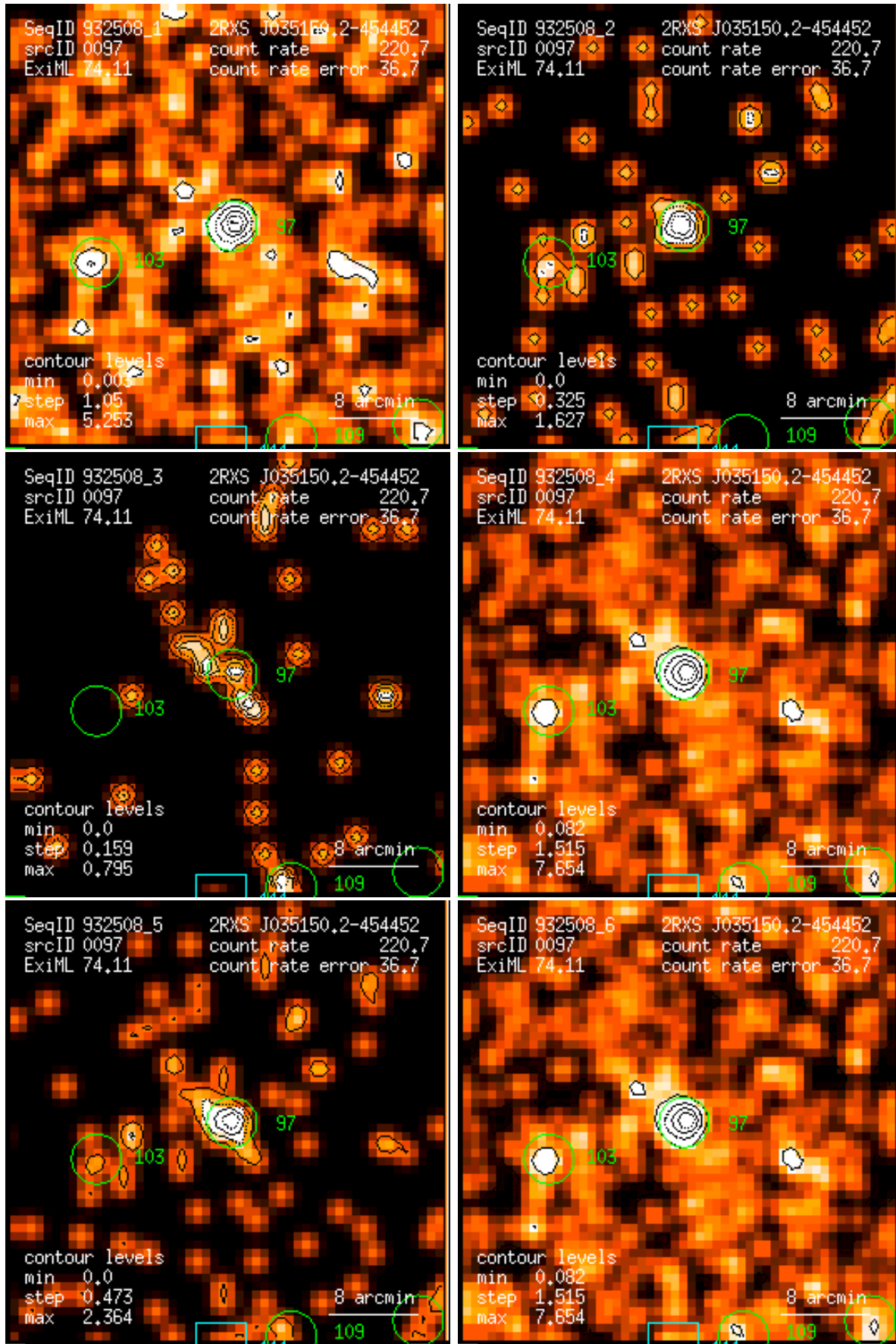
Figure 97: RASS 932508: detection 0097: band rate images, Gaussian filter: (1) PSPC channels 11 – 41, (2) 52 – 90, (3) 91 – 201, (4) 11 – 235, (5) 52 – 201, (6) 11 – 201. Broad band rates in counts/ks. Band rate contour levels in counts/ks/arcmin 2 .
