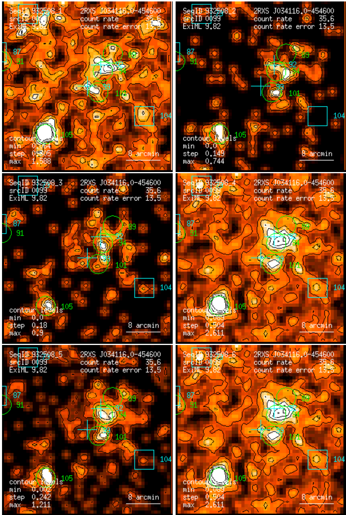
Figure 99: RASS 932508: detection 0099: band rate images, Gaussian filter: (1) PSPC channels 11 – 41, (2) 52 – 90, (3) 91 – 201, (4) 11 – 235, (5) 52 – 201, (6) 11 – 201. Broad band rates in counts/ks. Band rate contour levels in counts/ks/arcmin 2 .
