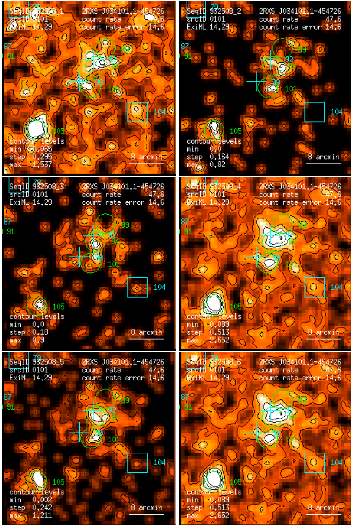
Figure 101: RASS 932508: detection 0101: band rate images, Gaussian filter: (1) PSPC channels 11 – 41, (2) 52 – 90, (3) 91 – 201, (4) 11 – 235, (5) 52 – 201, (6) 11 – 201. Broad band rates in counts/ks. Band rate contour levels in counts/ks/arcmin 2 .
