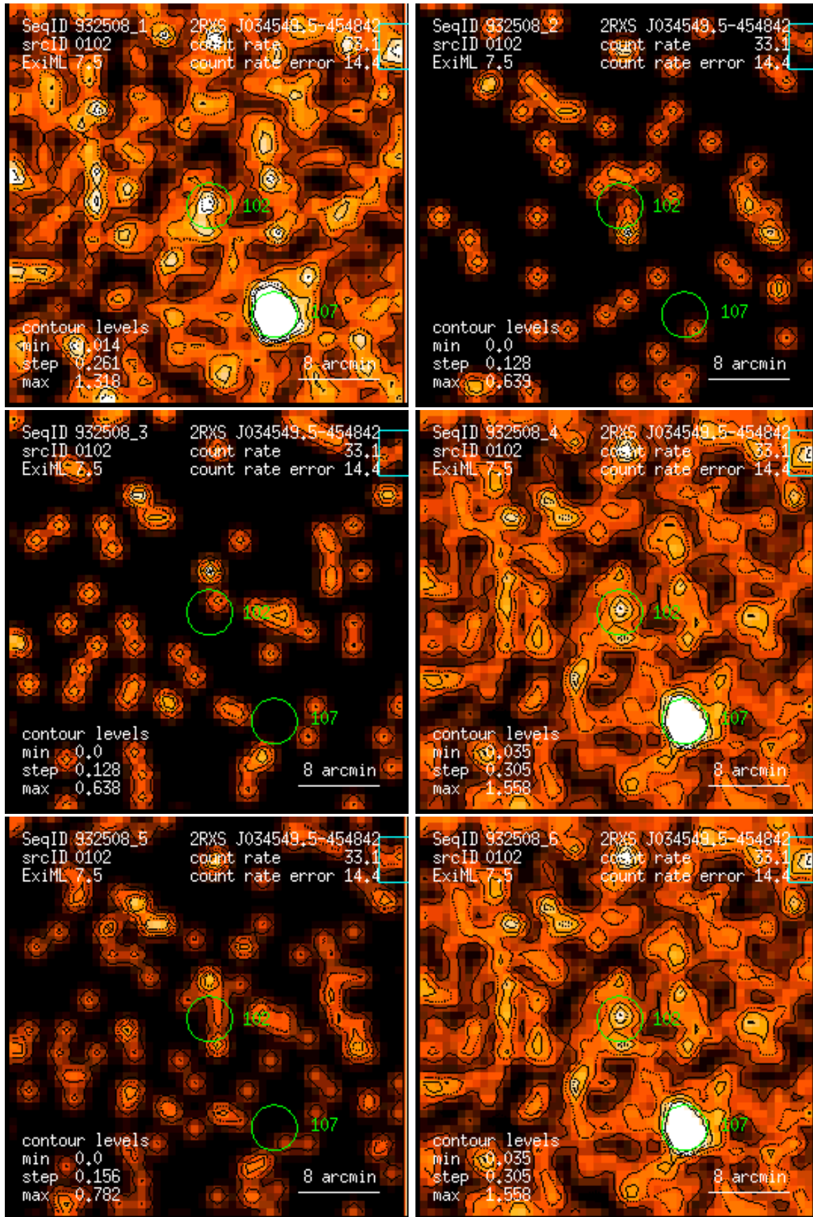
Figure 102: RASS 932508: detection 0102: band rate images, Gaussian filter: (1) PSPC channels 11 – 41, (2) 52 – 90, (3) 91 – 201, (4) 11 – 235, (5) 52 – 201, (6) 11 – 201. Broad band rates in counts/ks. Band rate contour levels in counts/ks/arcmin 2 .
