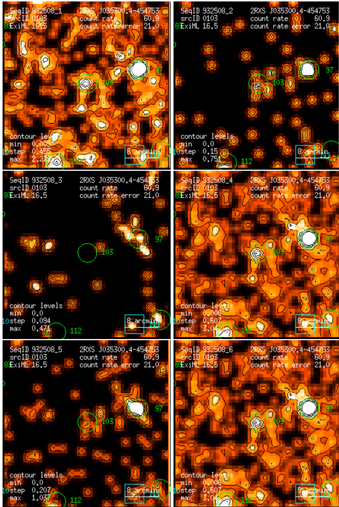
Figure 103: RASS 932508: detection 0103: band rate images, Gaussian filter: (1) PSPC channels 11 – 41, (2) 52 – 90, (3) 91 – 201, (4) 11 – 235, (5) 52 – 201, (6) 11 – 201. Broad band rates in counts/ks. Band rate contour levels in counts/ks/arcmin 2 .
