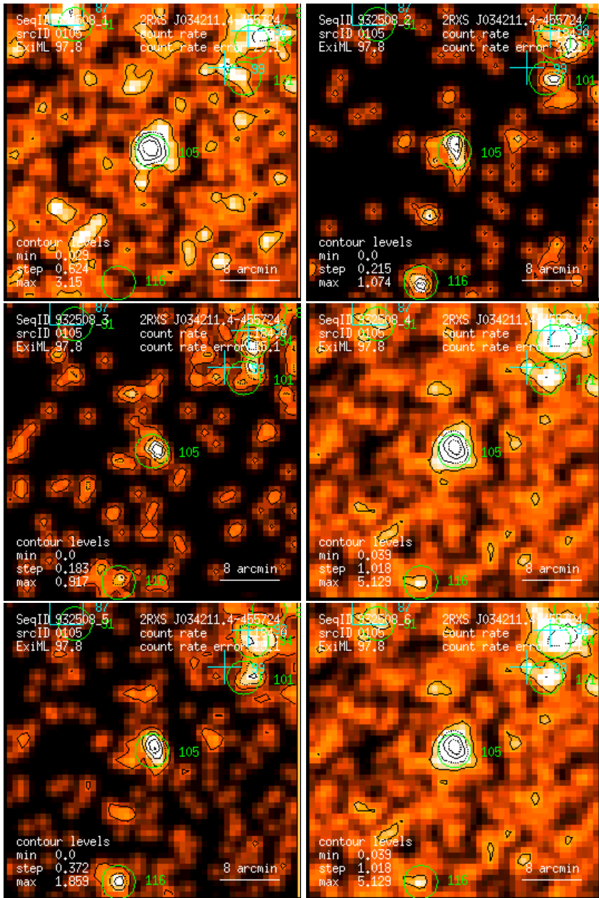
Figure 105: RASS 932508: detection 0105: band rate images, Gaussian filter: (1) PSPC channels 11 – 41, (2) 52 – 90, (3) 91 – 201, (4) 11 – 235, (5) 52 – 201, (6) 11 – 201. Broad band rates in counts/ks. Band rate contour levels in counts/ks/arcmin 2 .
