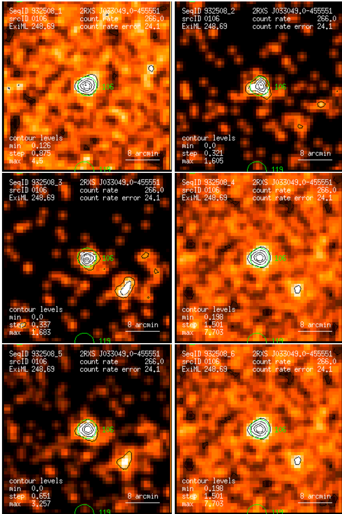
Figure 106: RASS 932508: detection 0106: band rate images, Gaussian filter: (1) PSPC channels 11 – 41, (2) 52 – 90, (3) 91 – 201, (4) 11 – 235, (5) 52 – 201, (6) 11 – 201. Broad band rates in counts/ks. Band rate contour levels in counts/ks/arcmin 2 .
