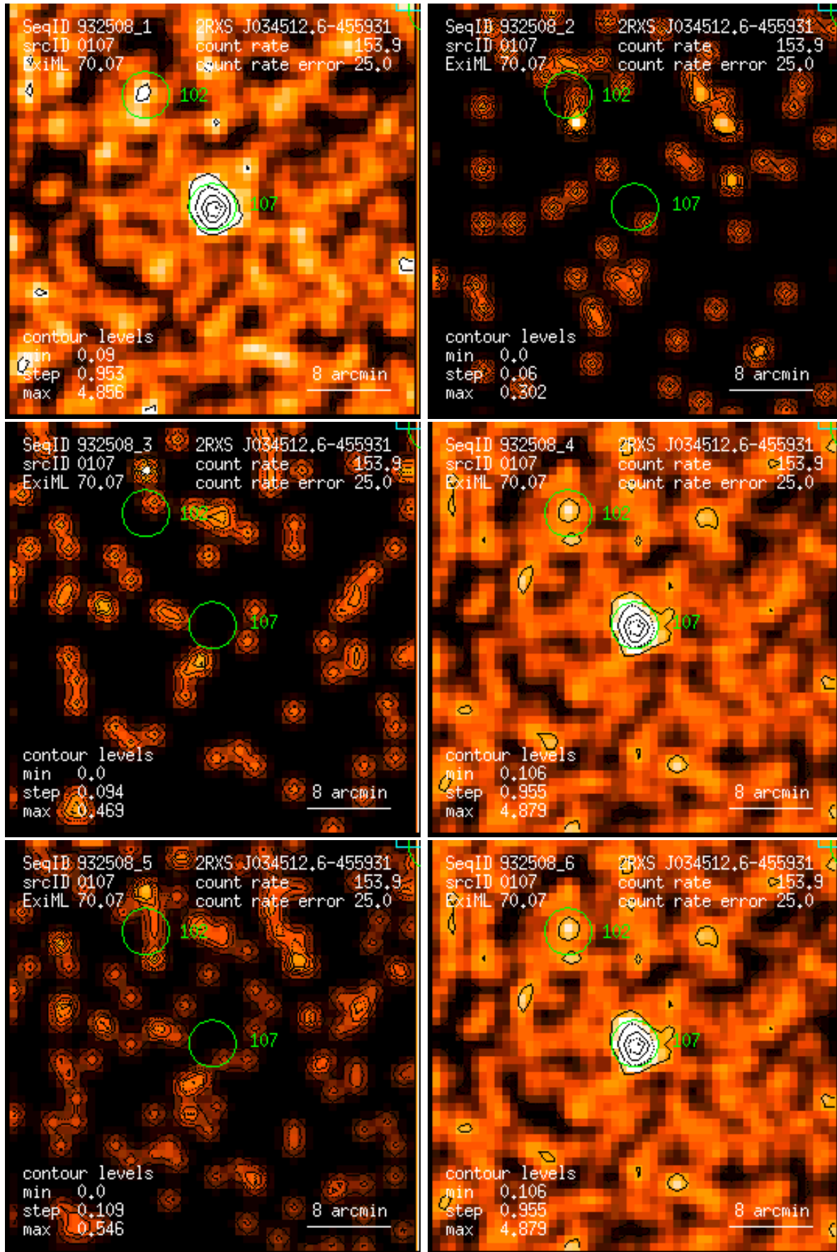
Figure 107: RASS 932508: detection 0107: band rate images, Gaussian filter: (1) PSPC channels 11 – 41, (2) 52 – 90, (3) 91 – 201, (4) 11 – 235, (5) 52 – 201, (6) 11 – 201. Broad band rates in counts/ks. Band rate contour levels in counts/ks/arcmin 2 .
