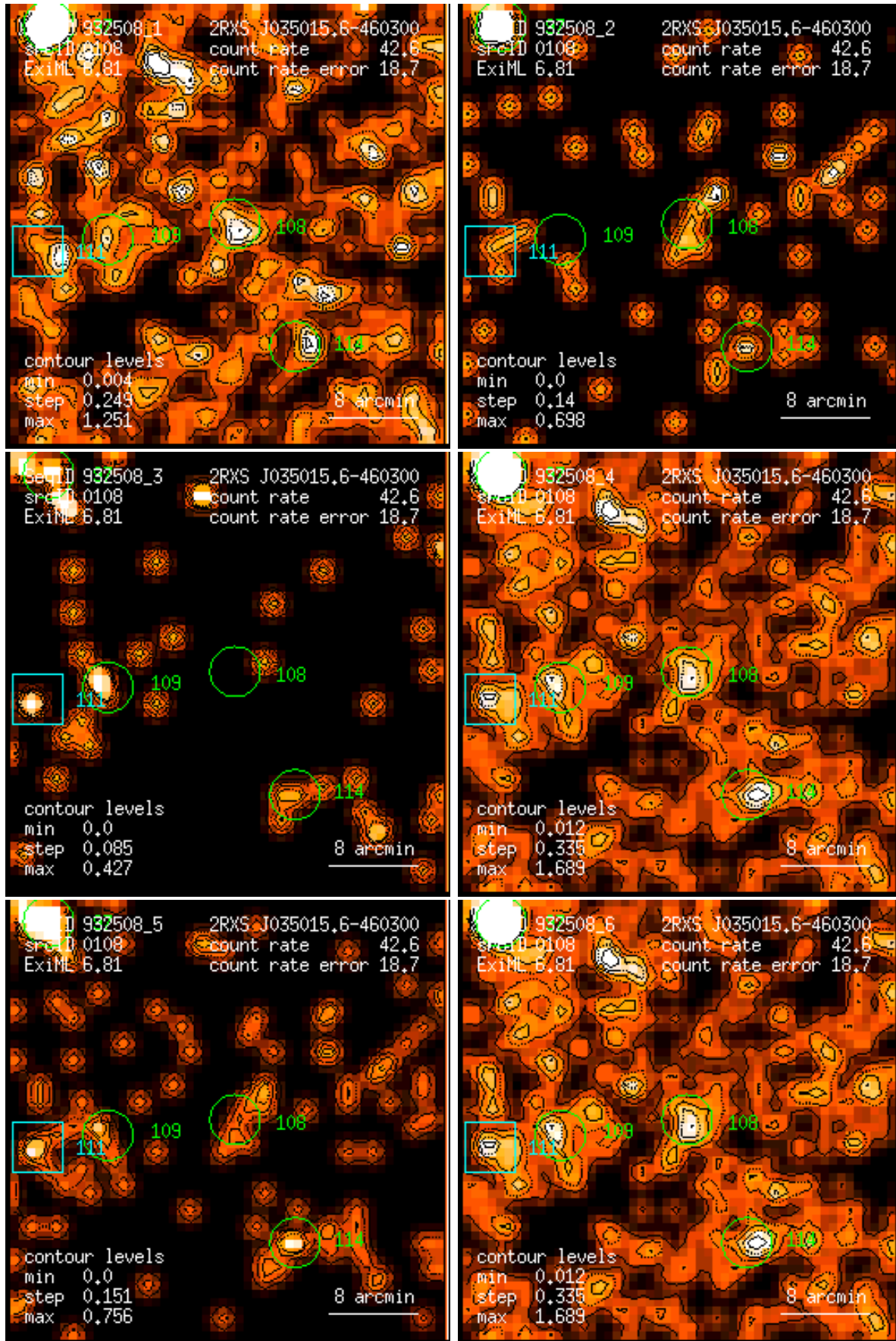
Figure 108: RASS 932508: detection 0108: band rate images, Gaussian filter: (1) PSPC channels 11 – 41, (2) 52 – 90, (3) 91 – 201, (4) 11 – 235, (5) 52 – 201, (6) 11 – 201. Broad band rates in counts/ks. Band rate contour levels in counts/ks/arcmin 2 .
