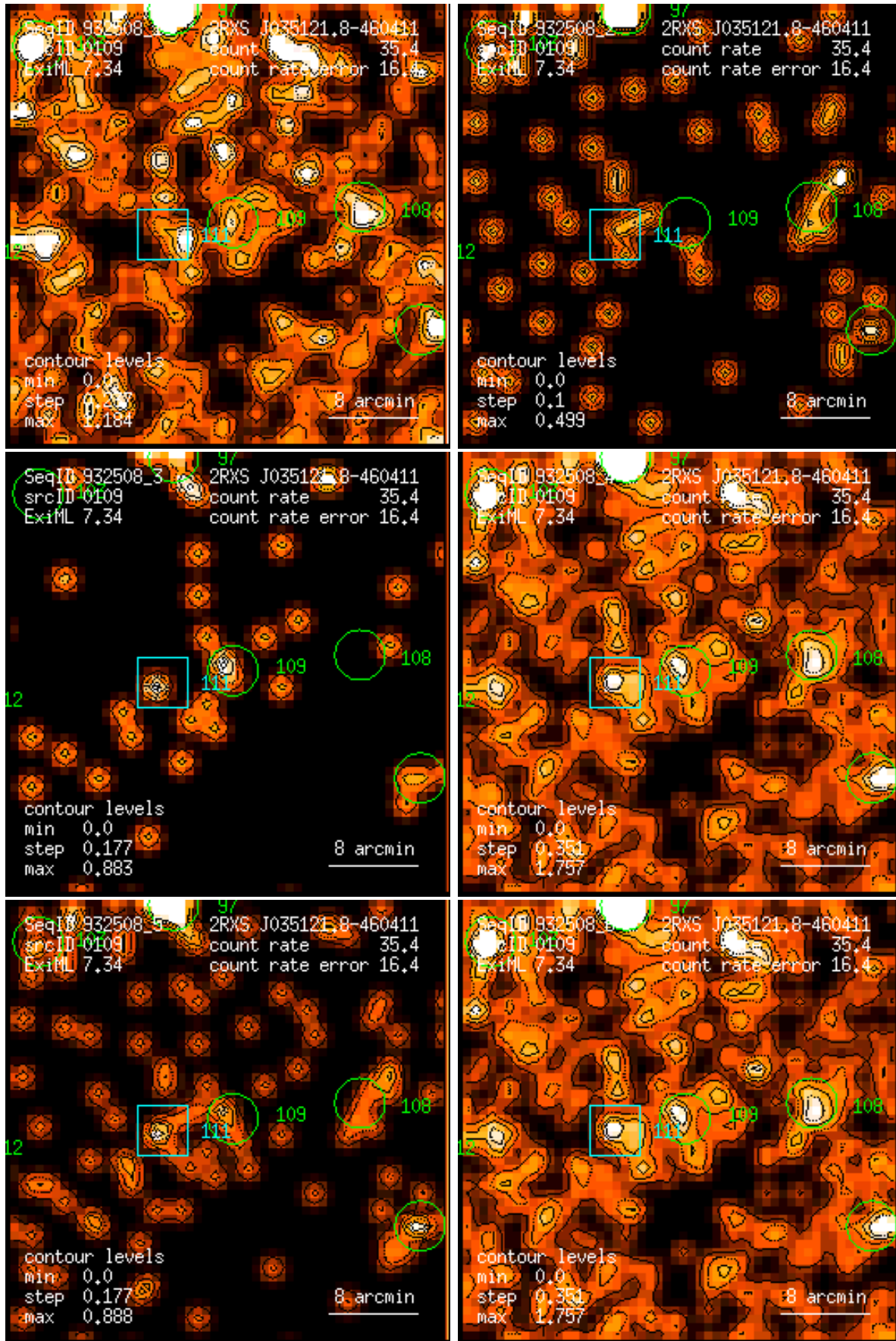
Figure 109: RASS 932508: detection 0109: band rate images, Gaussian filter: (1) PSPC channels 11 – 41, (2) 52 – 90, (3) 91 – 201, (4) 11 – 235, (5) 52 – 201, (6) 11 – 201. Broad band rates in counts/ks. Band rate contour levels in counts/ks/arcmin 2 .
