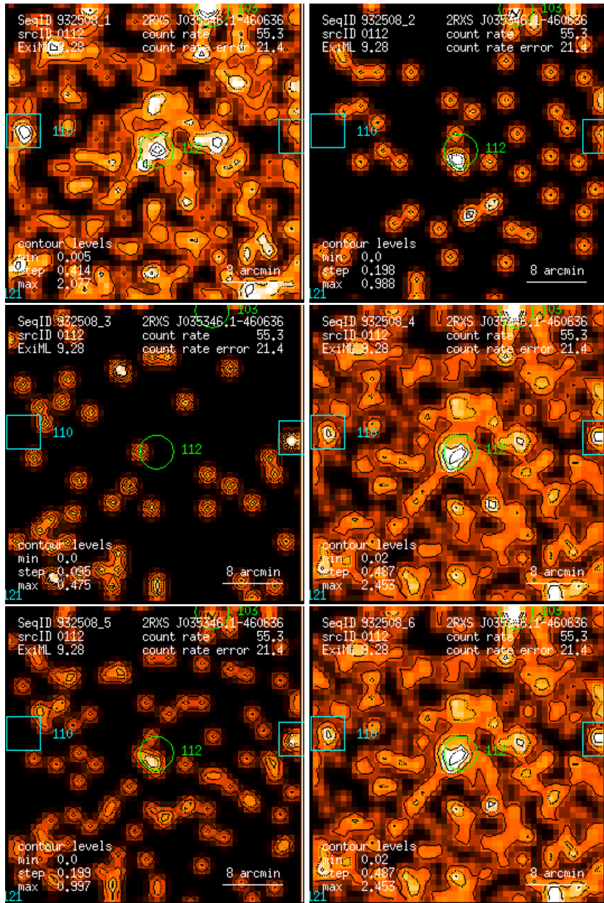
Figure 112: RASS 932508: detection 0112: band rate images, Gaussian filter: (1) PSPC channels 11 – 41, (2) 52 – 90, (3) 91 – 201, (4) 11 – 235, (5) 52 – 201, (6) 11 – 201. Broad band rates in counts/ks. Band rate contour levels in counts/ks/arcmin 2 .
