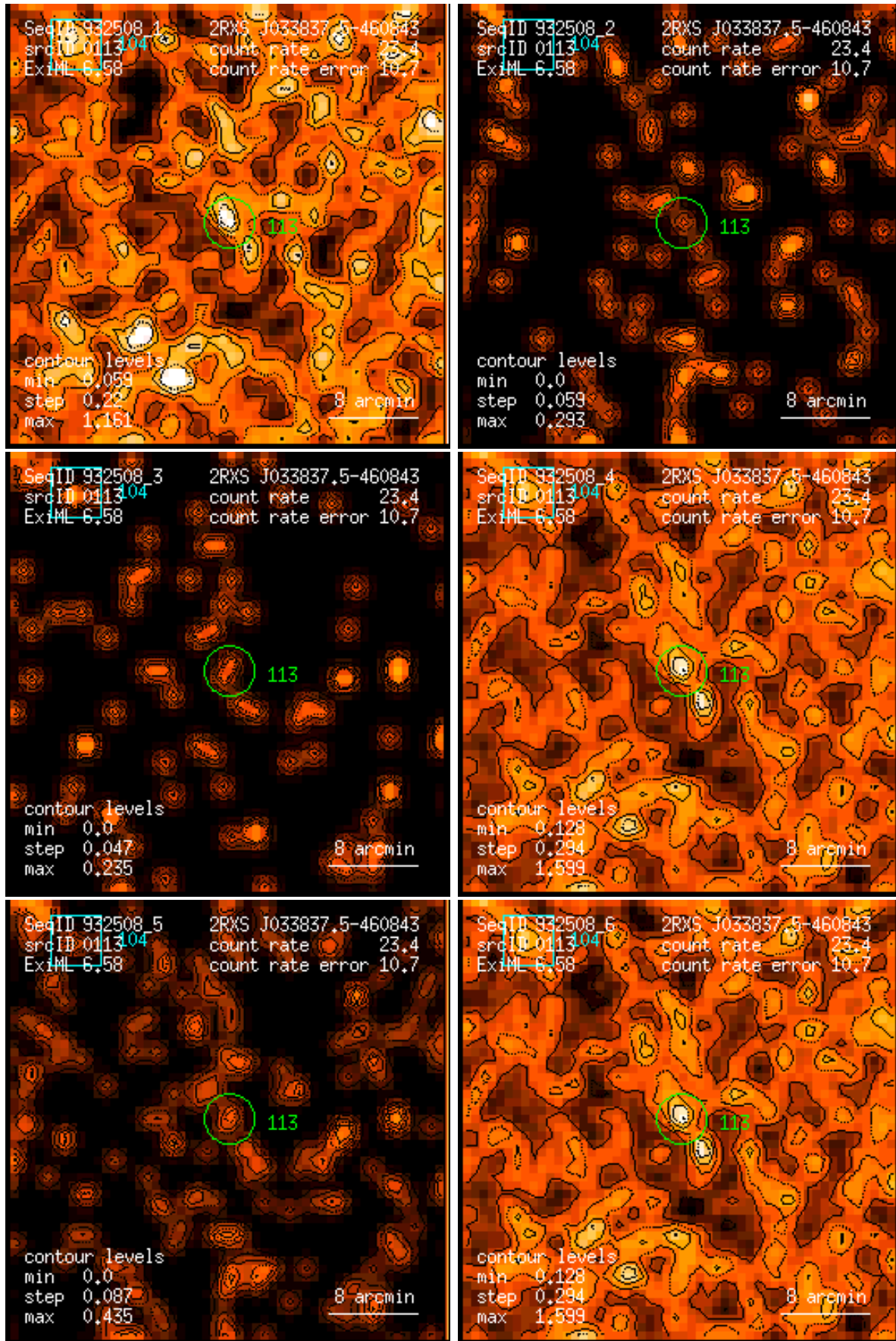
Figure 113: RASS 932508: detection 0113: band rate images, Gaussian filter: (1) PSPC channels 11 – 41, (2) 52 – 90, (3) 91 – 201, (4) 11 – 235, (5) 52 – 201, (6) 11 – 201. Broad band rates in counts/ks. Band rate contour levels in counts/ks/arcmin 2 .
