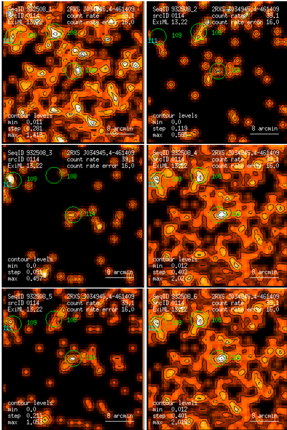
Figure 114: RASS 932508: detection 0114: band rate images, Gaussian filter: (1) PSPC channels 11 – 41, (2) 52 – 90, (3) 91 – 201, (4) 11 – 235, (5) 52 – 201, (6) 11 – 201. Broad band rates in counts/ks. Band rate contour levels in counts/ks/arcmin 2 .
