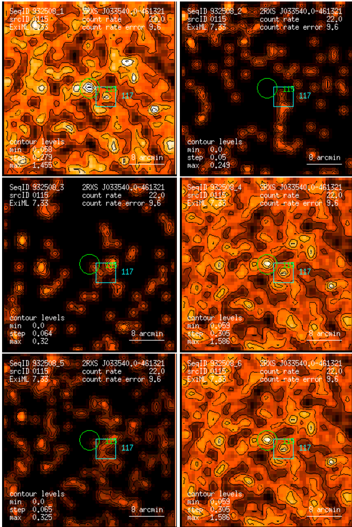
Figure 115: RASS 932508: detection 0115: band rate images, Gaussian filter: (1) PSPC channels 11 – 41, (2) 52 – 90, (3) 91 – 201, (4) 11 – 235, (5) 52 – 201, (6) 11 – 201. Broad band rates in counts/ks. Band rate contour levels in counts/ks/arcmin 2 .
