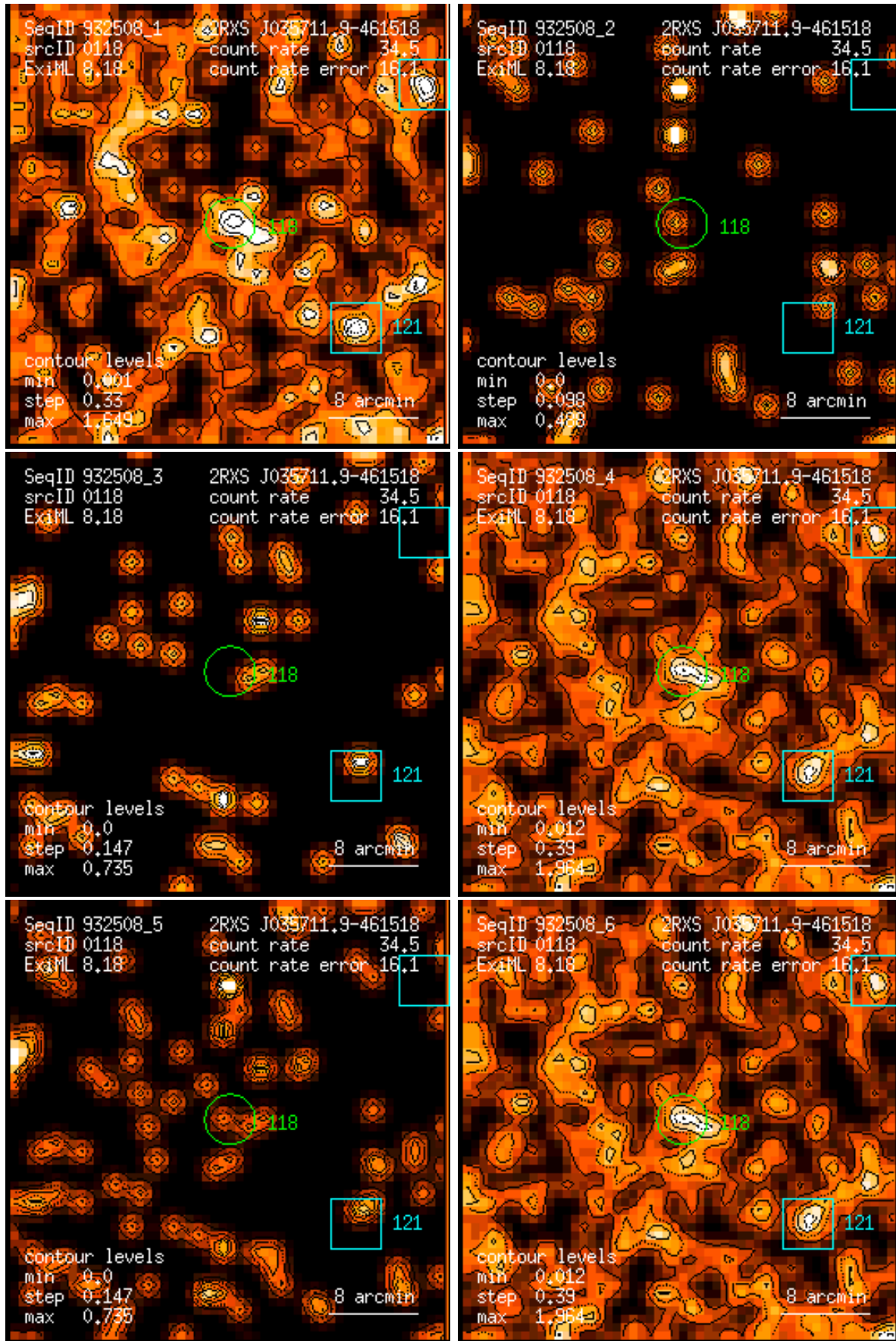
Figure 118: RASS 932508: detection 0118: band rate images, Gaussian filter: (1) PSPC channels 11 – 41, (2) 52 – 90, (3) 91 – 201, (4) 11 – 235, (5) 52 – 201, (6) 11 – 201. Broad band rates in counts/ks. Band rate contour levels in counts/ks/arcmin 2 .
