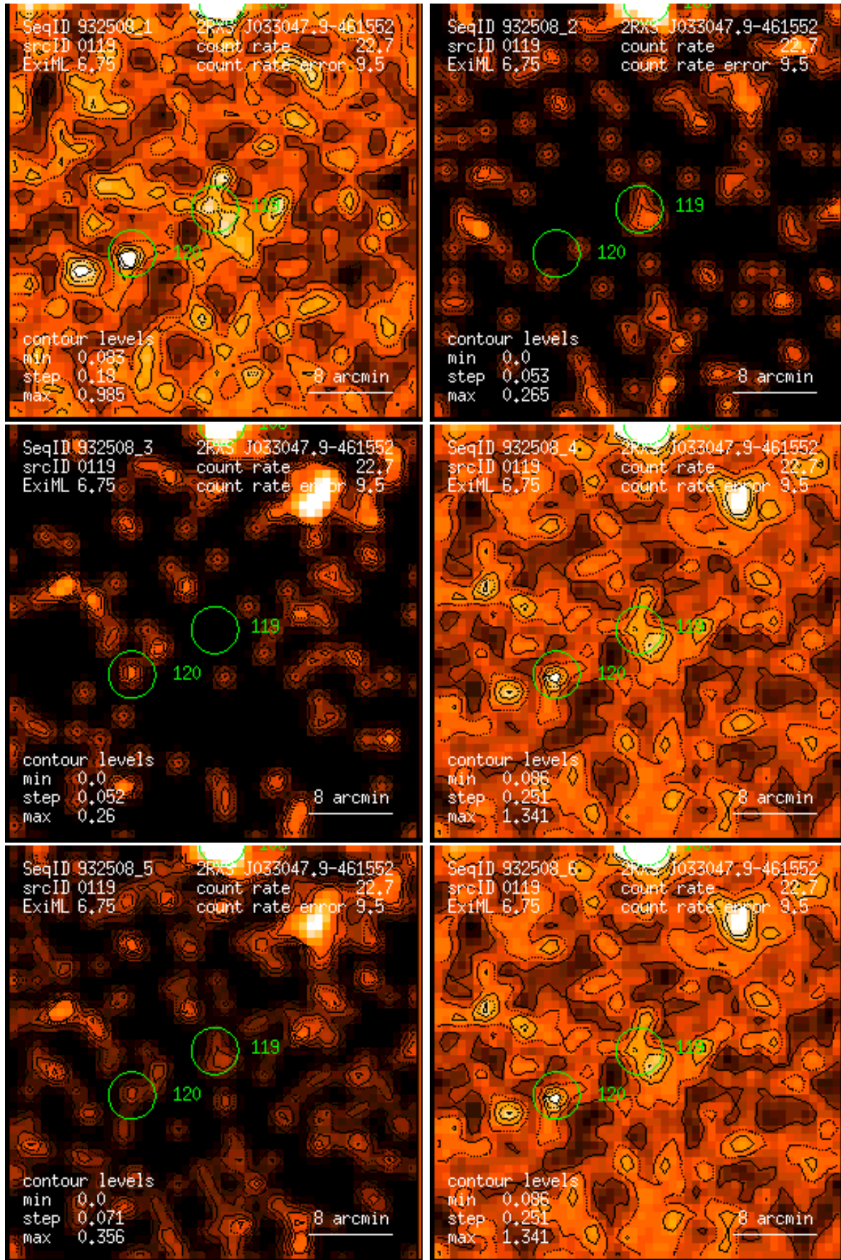
Figure 119: RASS 932508: detection 0119: band rate images, Gaussian filter: (1) PSPC channels 11 – 41, (2) 52 – 90, (3) 91 – 201, (4) 11 – 235, (5) 52 – 201, (6) 11 – 201. Broad band rates in counts/ks. Band rate contour levels in counts/ks/arcmin 2 .
