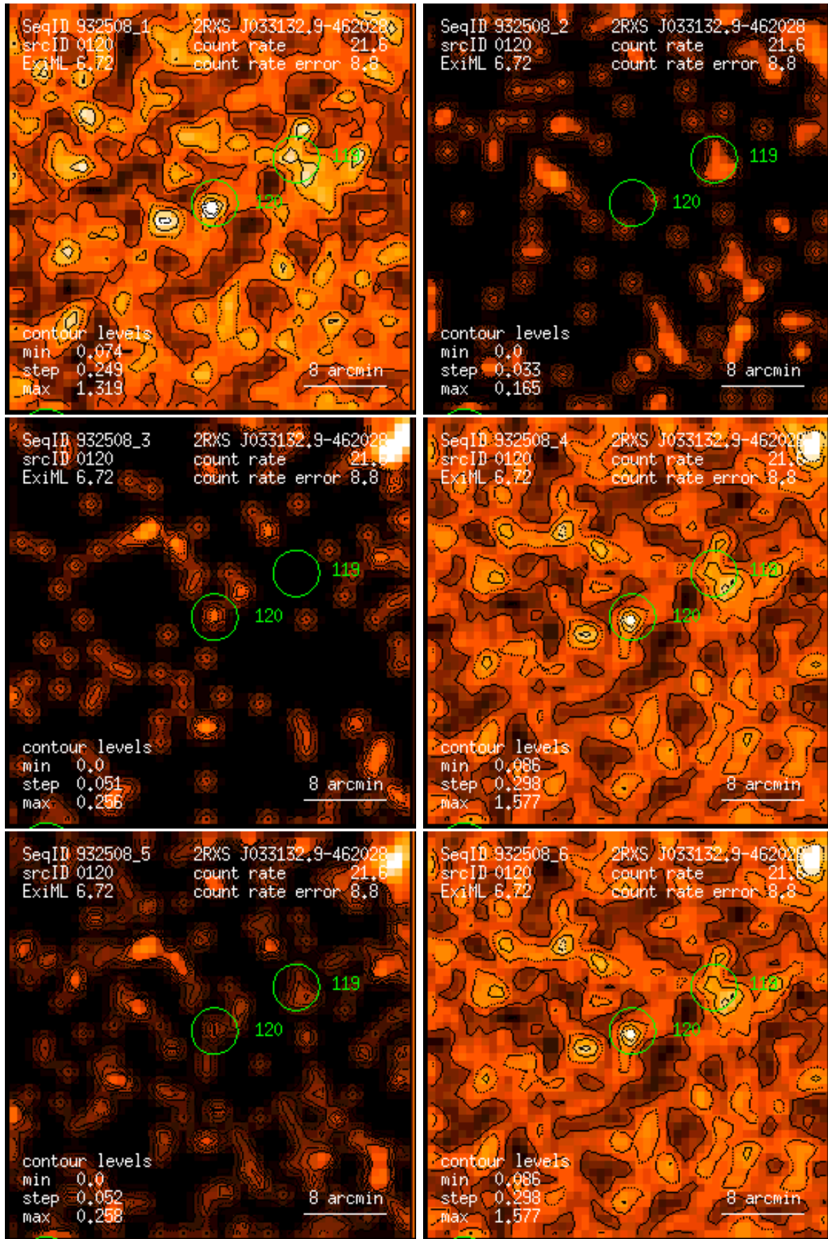
Figure 120: RASS 932508: detection 0120: band rate images, Gaussian filter: (1) PSPC channels 11 – 41, (2) 52 – 90, (3) 91 – 201, (4) 11 – 235, (5) 52 – 201, (6) 11 – 201. Broad band rates in counts/ks. Band rate contour levels in counts/ks/arcmin 2 .
