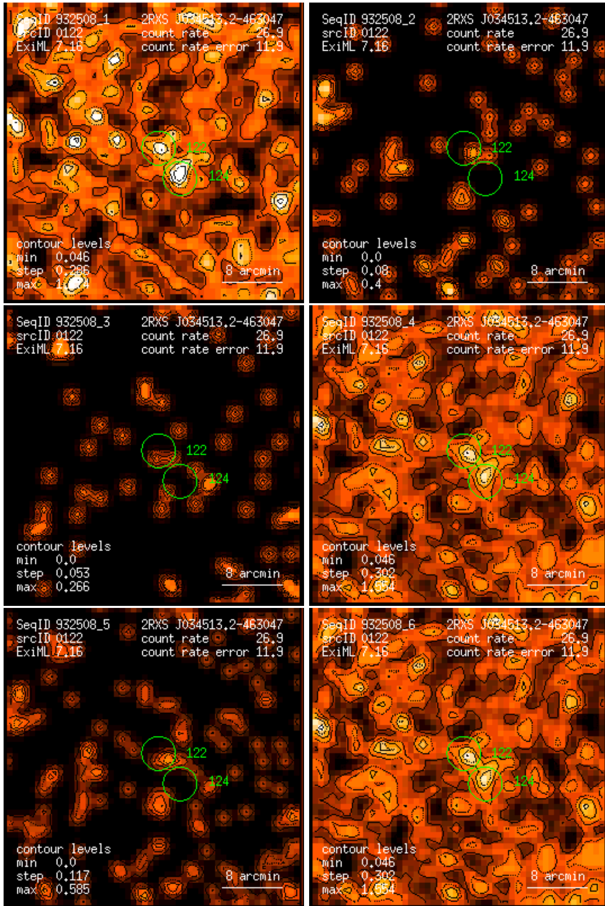
Figure 122: RASS 932508: detection 0122: band rate images, Gaussian filter: (1) PSPC channels 11 – 41, (2) 52 – 90, (3) 91 – 201, (4) 11 – 235, (5) 52 – 201, (6) 11 – 201. Broad band rates in counts/ks. Band rate contour levels in counts/ks/arcmin 2 .
