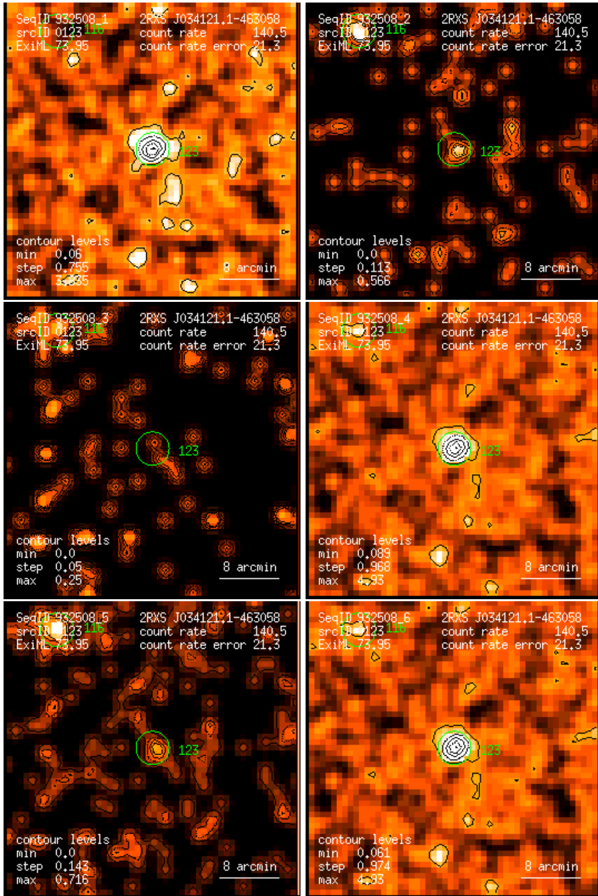
Figure 123: RASS 932508: detection 0123: band rate images, Gaussian filter: (1) PSPC channels 11 – 41, (2) 52 – 90, (3) 91 – 201, (4) 11 – 235, (5) 52 – 201, (6) 11 – 201. Broad band rates in counts/ks. Band rate contour levels in counts/ks/arcmin 2 .
