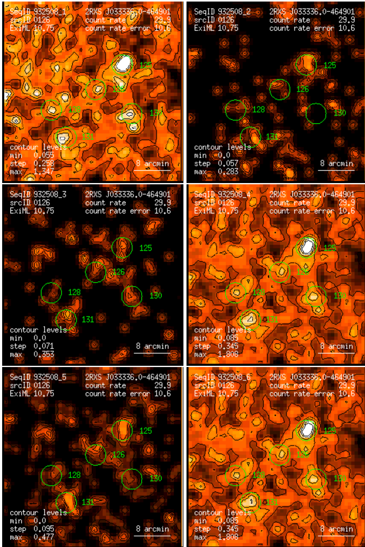
Figure 126: RASS 932508: detection 0126: band rate images, Gaussian filter: (1) PSPC channels 11 – 41, (2) 52 – 90, (3) 91 – 201, (4) 11 – 235, (5) 52 – 201, (6) 11 – 201. Broad band rates in counts/ks. Band rate contour levels in counts/ks/arcmin 2 .
