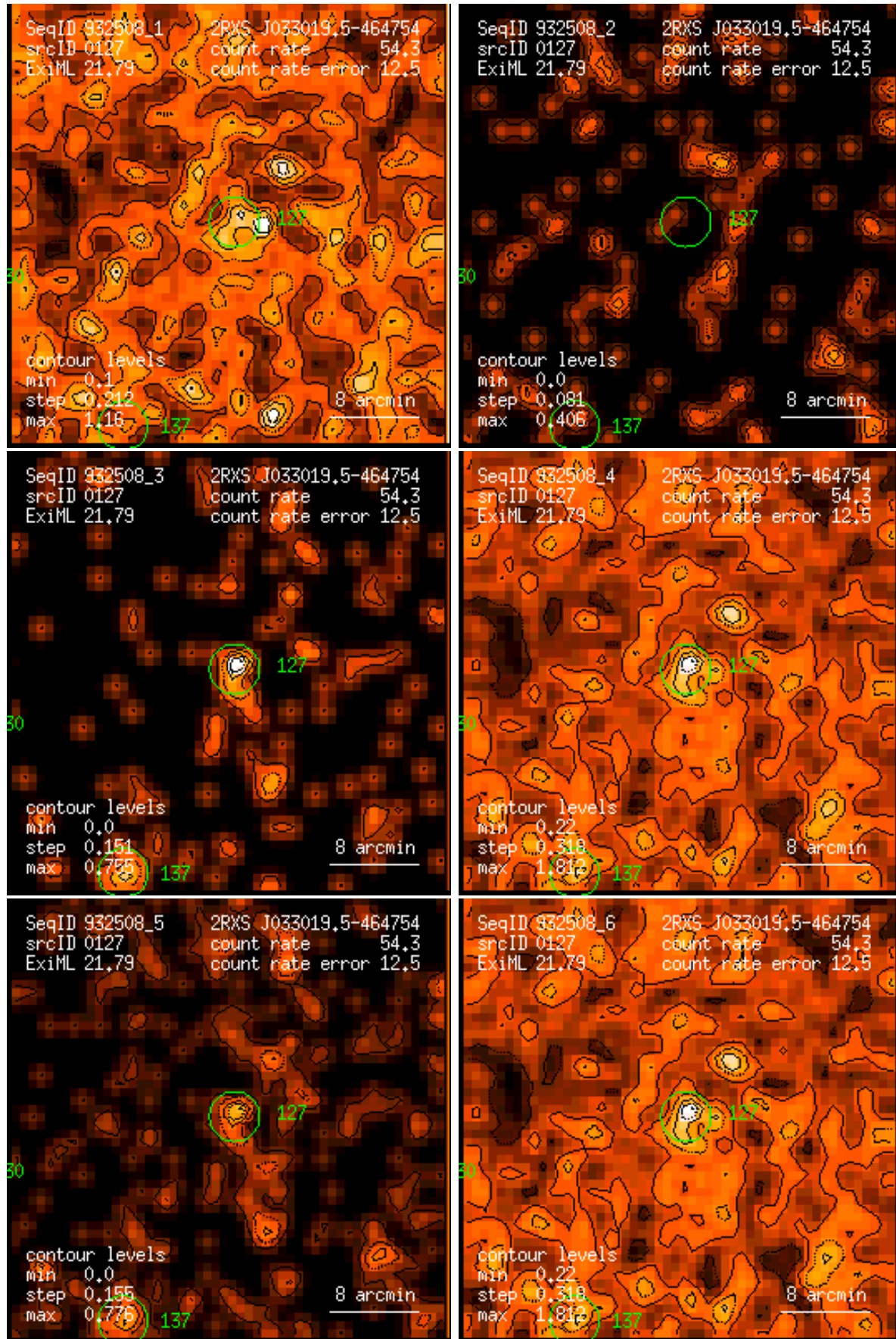
Figure 127: RASS 932508: detection 0127: band rate images, Gaussian filter: (1) PSPC channels 11 – 41, (2) 52 – 90, (3) 91 – 201, (4) 11 – 235, (5) 52 – 201, (6) 11 – 201. Broad band rates in counts/ks. Band rate contour levels in counts/ks/arcmin 2 .
