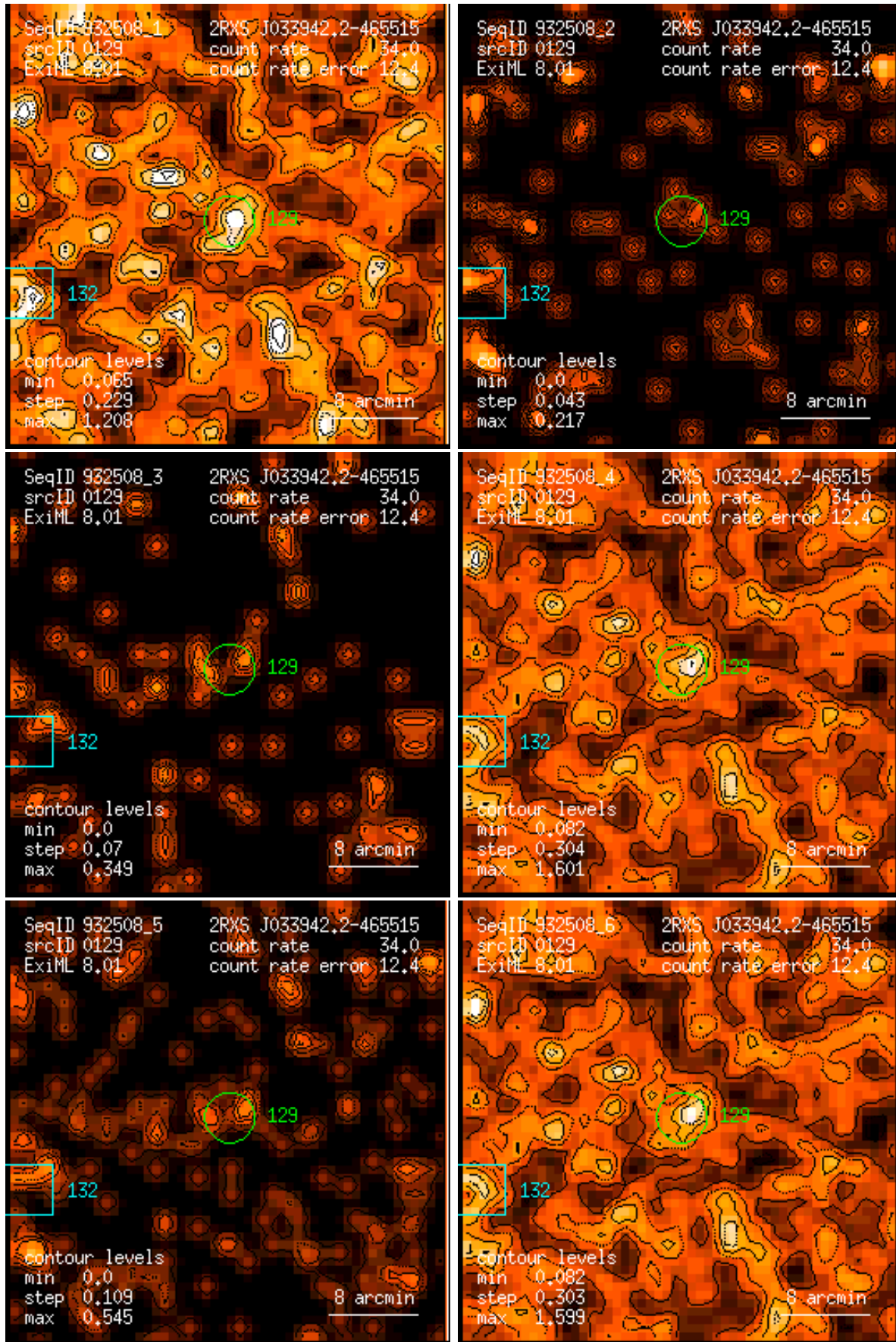
Figure 129: RASS 932508: detection 0129: band rate images, Gaussian filter: (1) PSPC channels 11 – 41, (2) 52 – 90, (3) 91 – 201, (4) 11 – 235, (5) 52 – 201, (6) 11 – 201. Broad band rates in counts/ks. Band rate contour levels in counts/ks/arcmin 2 .
