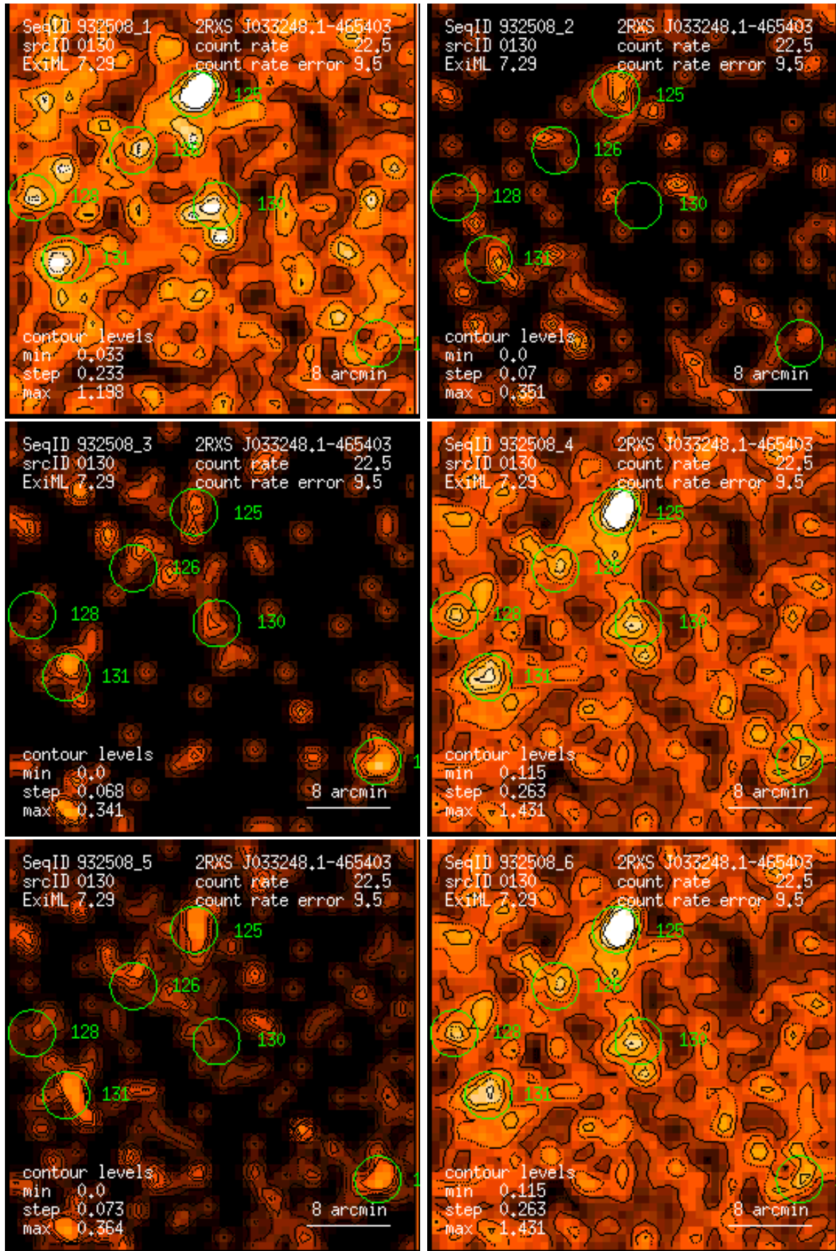
Figure 130: RASS 932508: detection 0130: band rate images, Gaussian filter: (1) PSPC channels 11 – 41, (2) 52 – 90, (3) 91 – 201, (4) 11 – 235, (5) 52 – 201, (6) 11 – 201. Broad band rates in counts/ks. Band rate contour levels in counts/ks/arcmin 2 .
