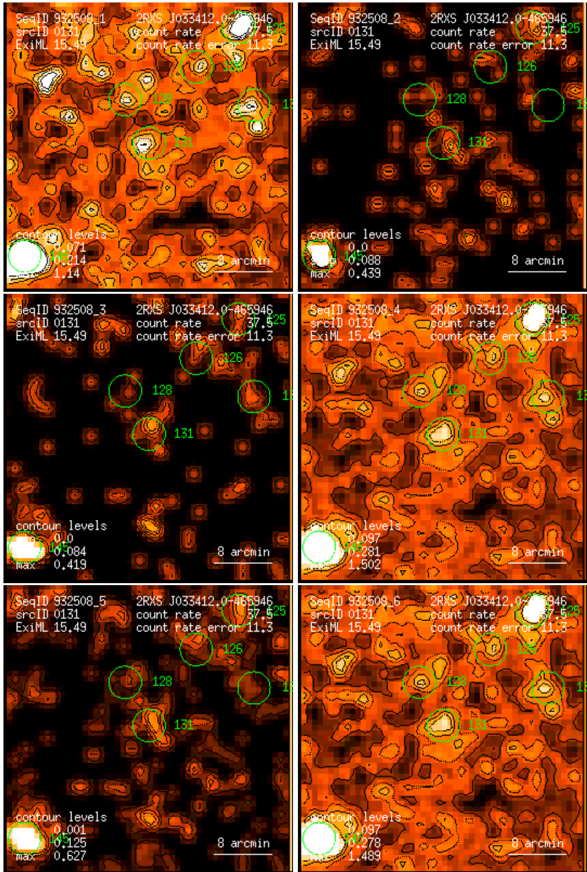
Figure 131: RASS 932508: detection 0131: band rate images, Gaussian filter: (1) PSPC channels 11 – 41, (2) 52 – 90, (3) 91 – 201, (4) 11 – 235, (5) 52 – 201, (6) 11 – 201. Broad band rates in counts/ks. Band rate contour levels in counts/ks/arcmin 2 .
