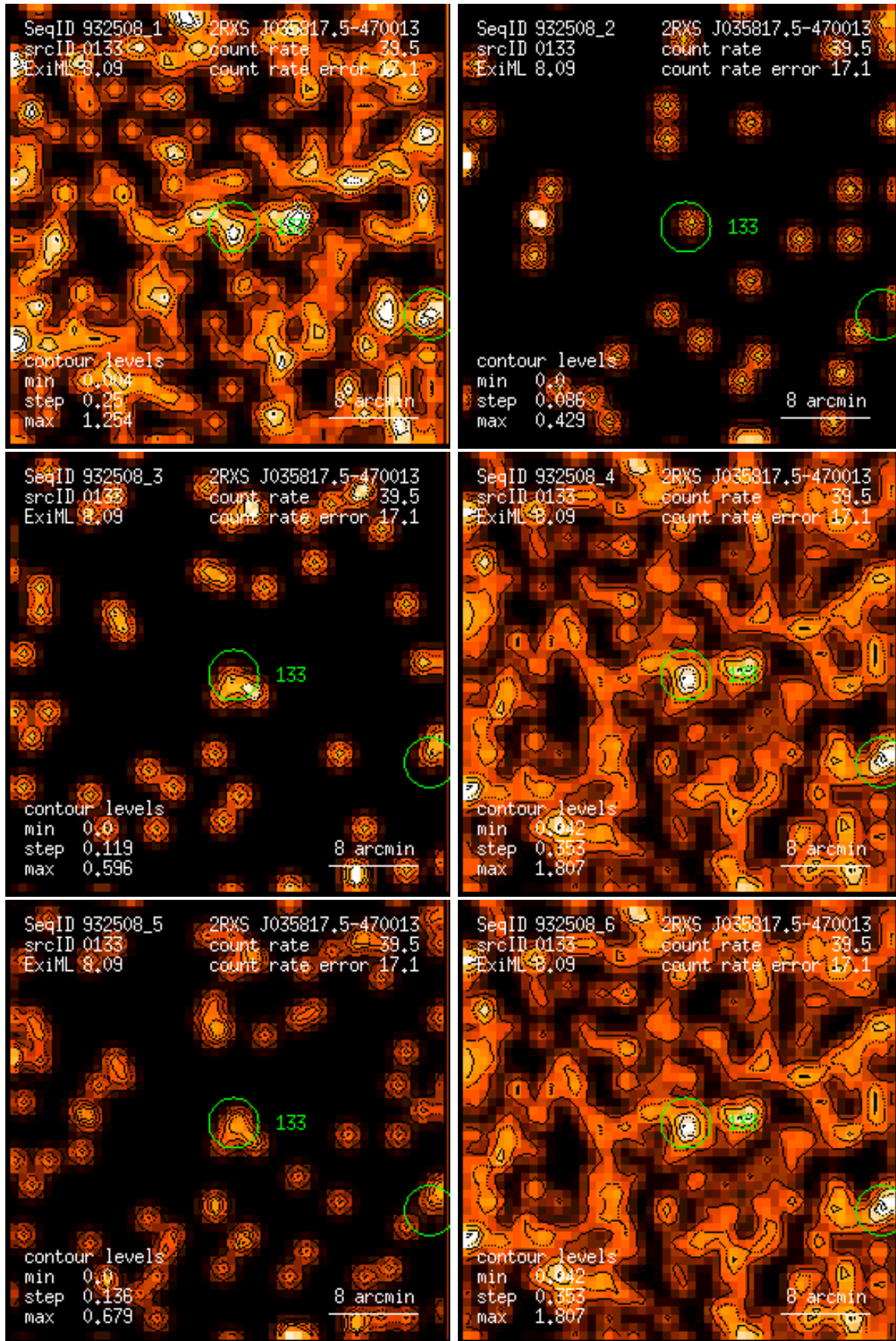
Figure 133: RASS 932508: detection 0133: band rate images, Gaussian filter: (1) PSPC channels 11 – 41, (2) 52 – 90, (3) 91 – 201, (4) 11 – 235, (5) 52 – 201, (6) 11 – 201. Broad band rates in counts/ks. Band rate contour levels in counts/ks/arcmin 2 .
