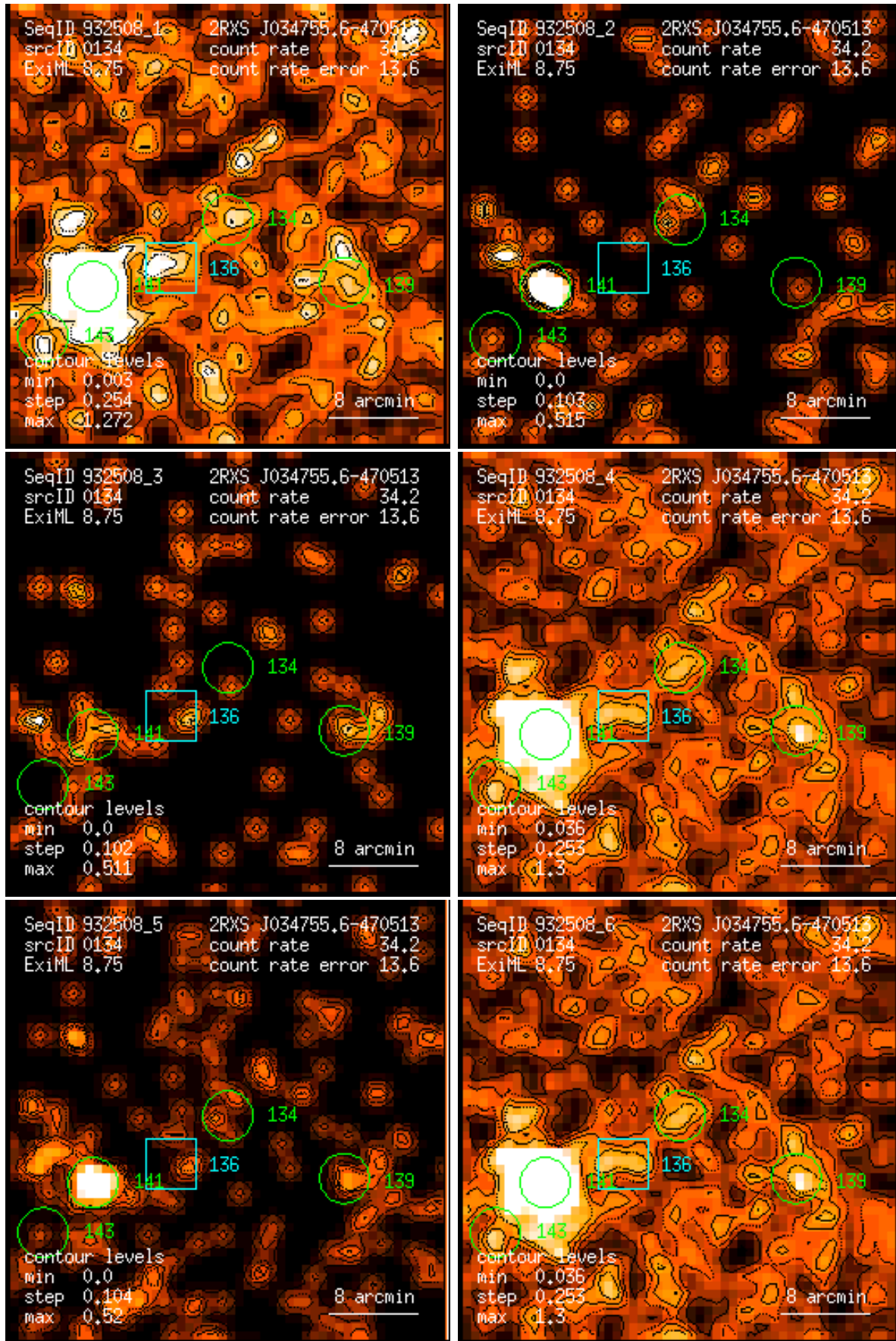
Figure 134: RASS 932508: detection 0134: band rate images, Gaussian filter: (1) PSPC channels 11 – 41, (2) 52 – 90, (3) 91 – 201, (4) 11 – 235, (5) 52 – 201, (6) 11 – 201. Broad band rates in counts/ks. Band rate contour levels in counts/ks/arcmin 2 .
