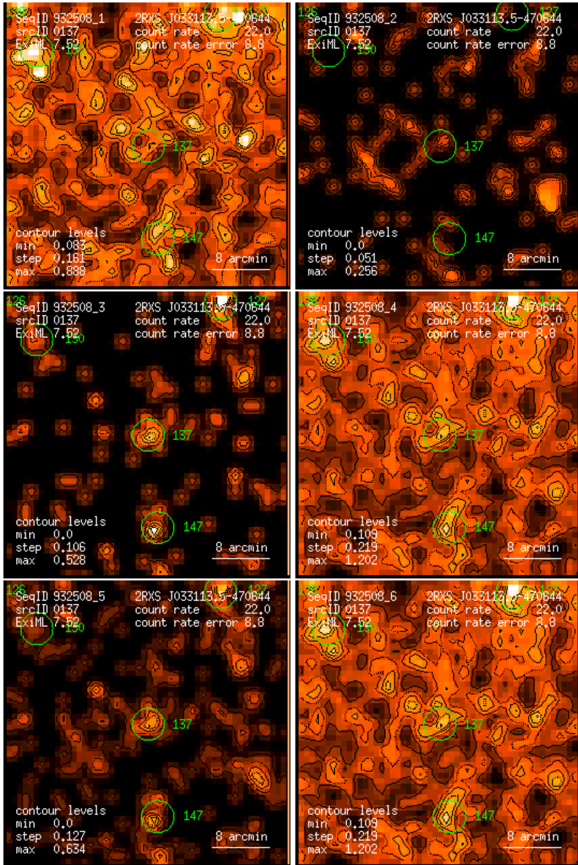
Figure 137: RASS 932508: detection 0137: band rate images, Gaussian filter: (1) PSPC channels 11 – 41, (2) 52 – 90, (3) 91 – 201, (4) 11 – 235, (5) 52 – 201, (6) 11 – 201. Broad band rates in counts/ks. Band rate contour levels in counts/ks/arcmin 2 .
