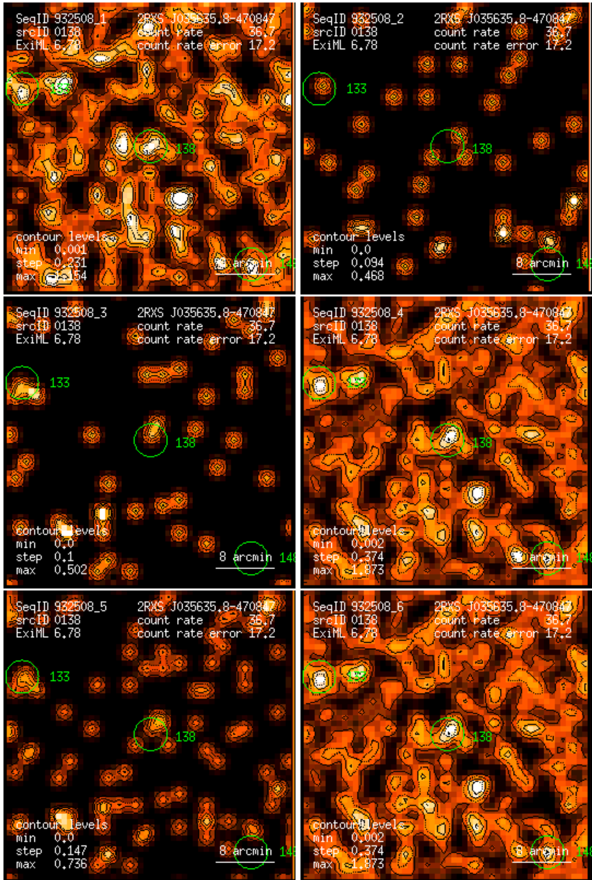
Figure 138: RASS 932508: detection 0138: band rate images, Gaussian filter: (1) PSPC channels 11 – 41, (2) 52 – 90, (3) 91 – 201, (4) 11 – 235, (5) 52 – 201, (6) 11 – 201. Broad band rates in counts/ks. Band rate contour levels in counts/ks/arcmin 2 .
