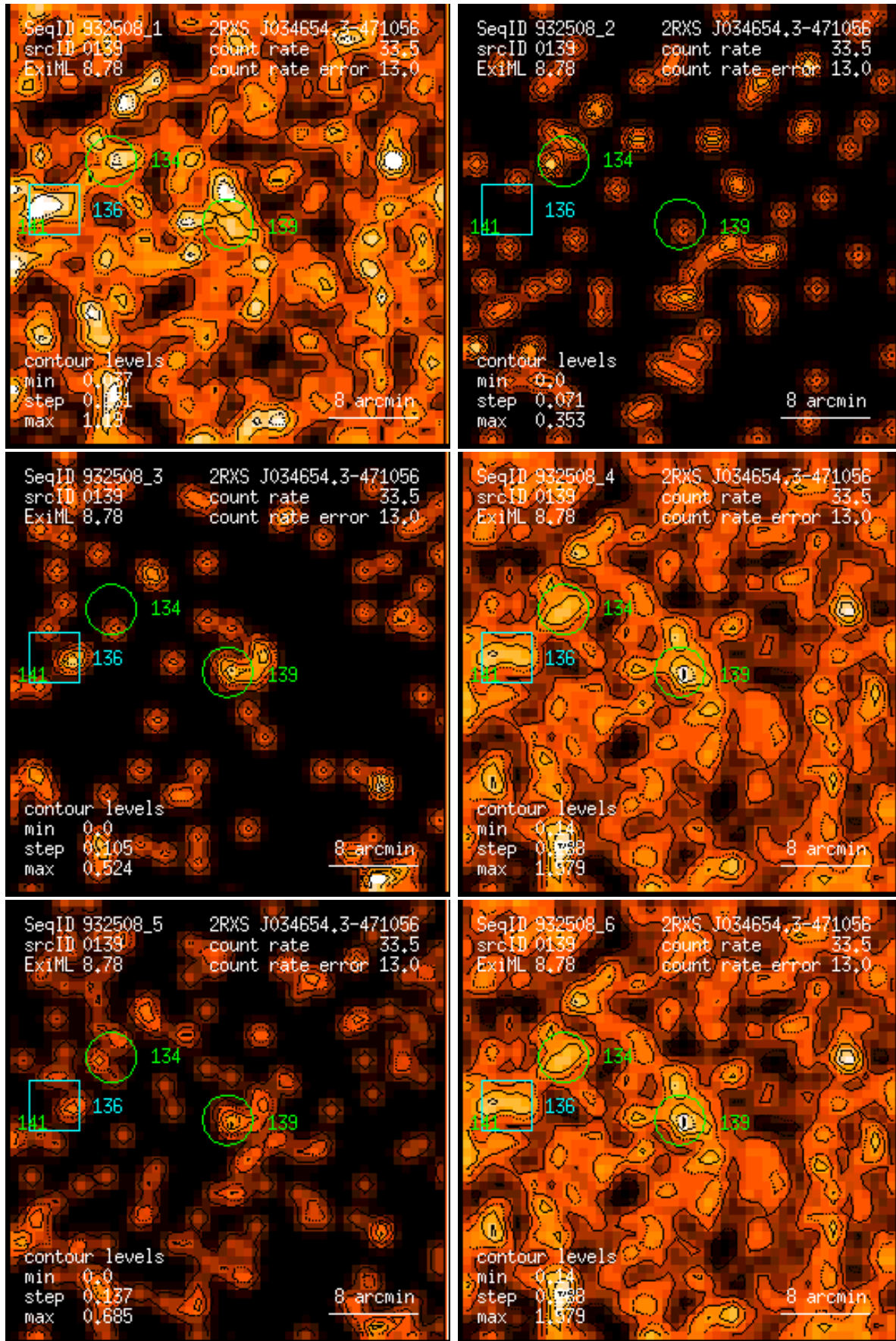
Figure 139: RASS 932508: detection 0139: band rate images, Gaussian filter: (1) PSPC channels 11 – 41, (2) 52 – 90, (3) 91 – 201, (4) 11 – 235, (5) 52 – 201, (6) 11 – 201. Broad band rates in counts/ks. Band rate contour levels in counts/ks/arcmin 2 .
