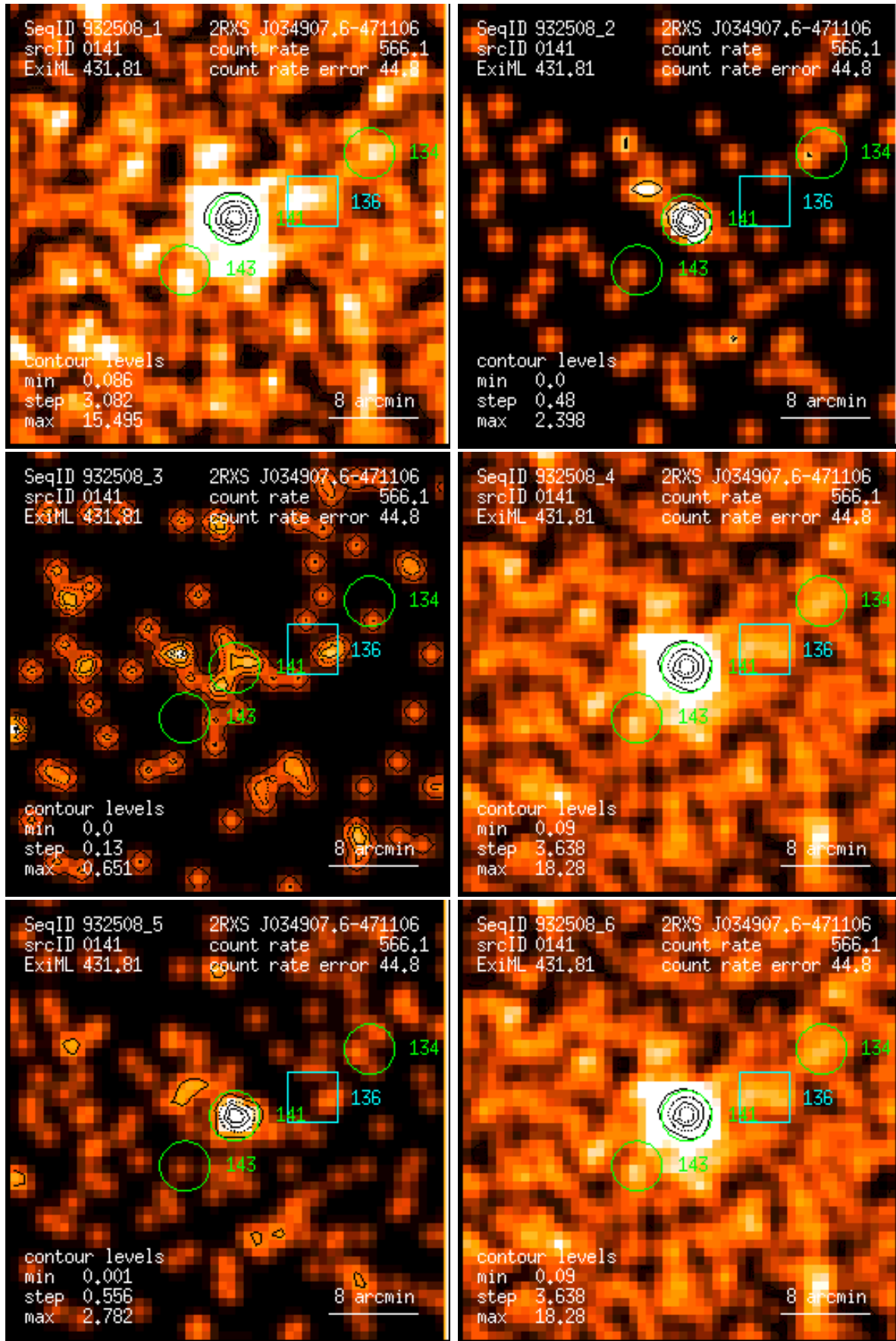
Figure 141: RASS 932508: detection 0141: band rate images, Gaussian filter: (1) PSPC channels 11 – 41, (2) 52 – 90, (3) 91 – 201, (4) 11 – 235, (5) 52 – 201, (6) 11 – 201. Broad band rates in counts/ks. Band rate contour levels in counts/ks/arcmin 2 .
