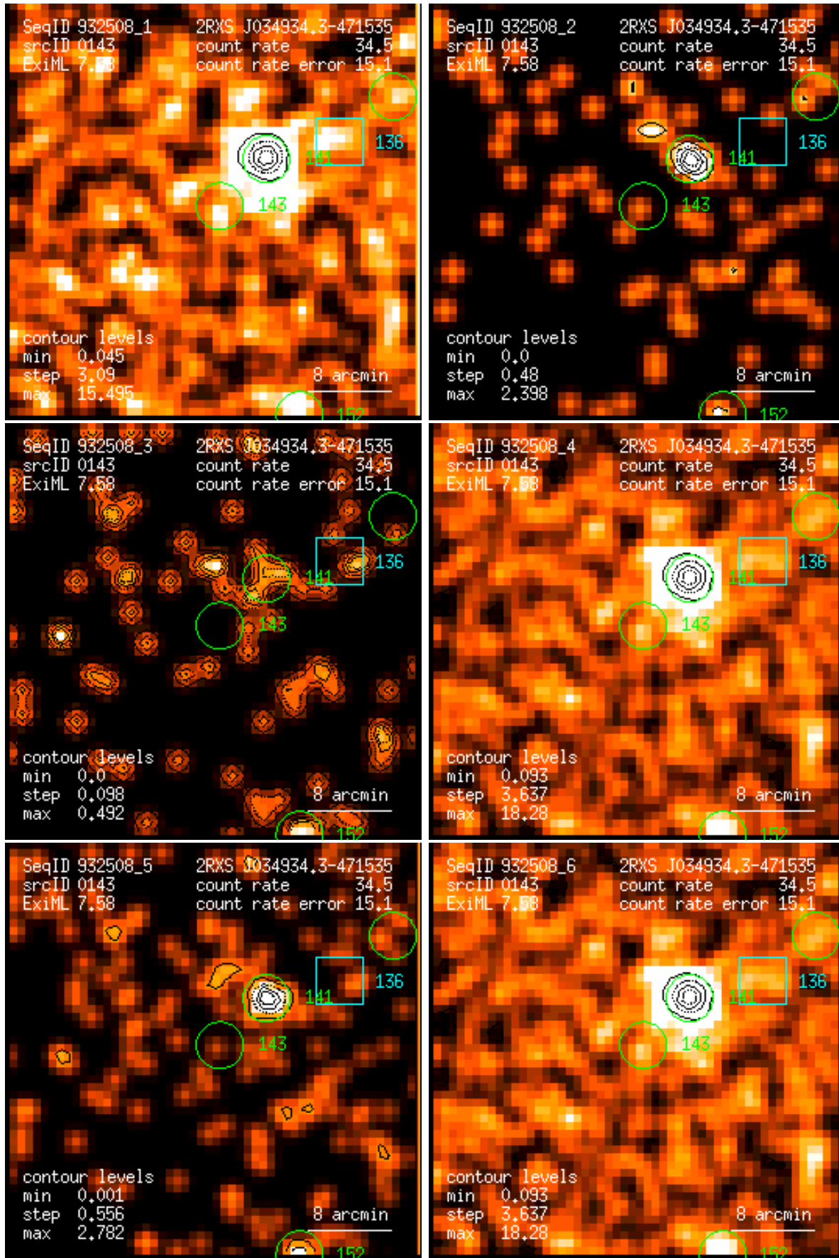
Figure 143: RASS 932508: detection 0143: band rate images, Gaussian filter: (1) PSPC channels 11 – 41, (2) 52 – 90, (3) 91 – 201, (4) 11 – 235, (5) 52 – 201, (6) 11 – 201. Broad band rates in counts/ks. Band rate contour levels in counts/ks/arcmin 2 .
