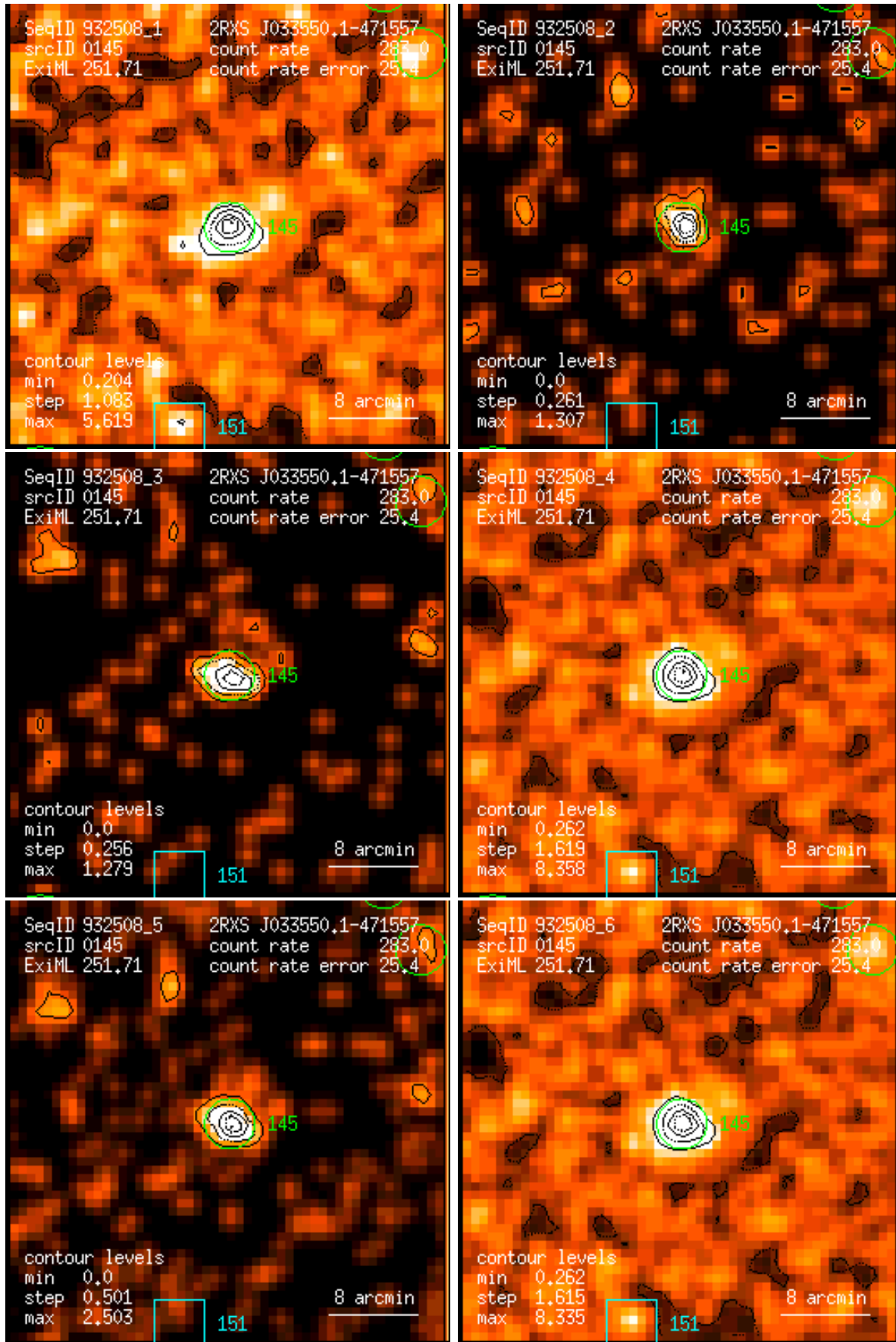
Figure 145: RASS 932508: detection 0145: band rate images, Gaussian filter: (1) PSPC channels 11 – 41, (2) 52 – 90, (3) 91 – 201, (4) 11 – 235, (5) 52 – 201, (6) 11 – 201. Broad band rates in counts/ks. Band rate contour levels in counts/ks/arcmin 2 .
