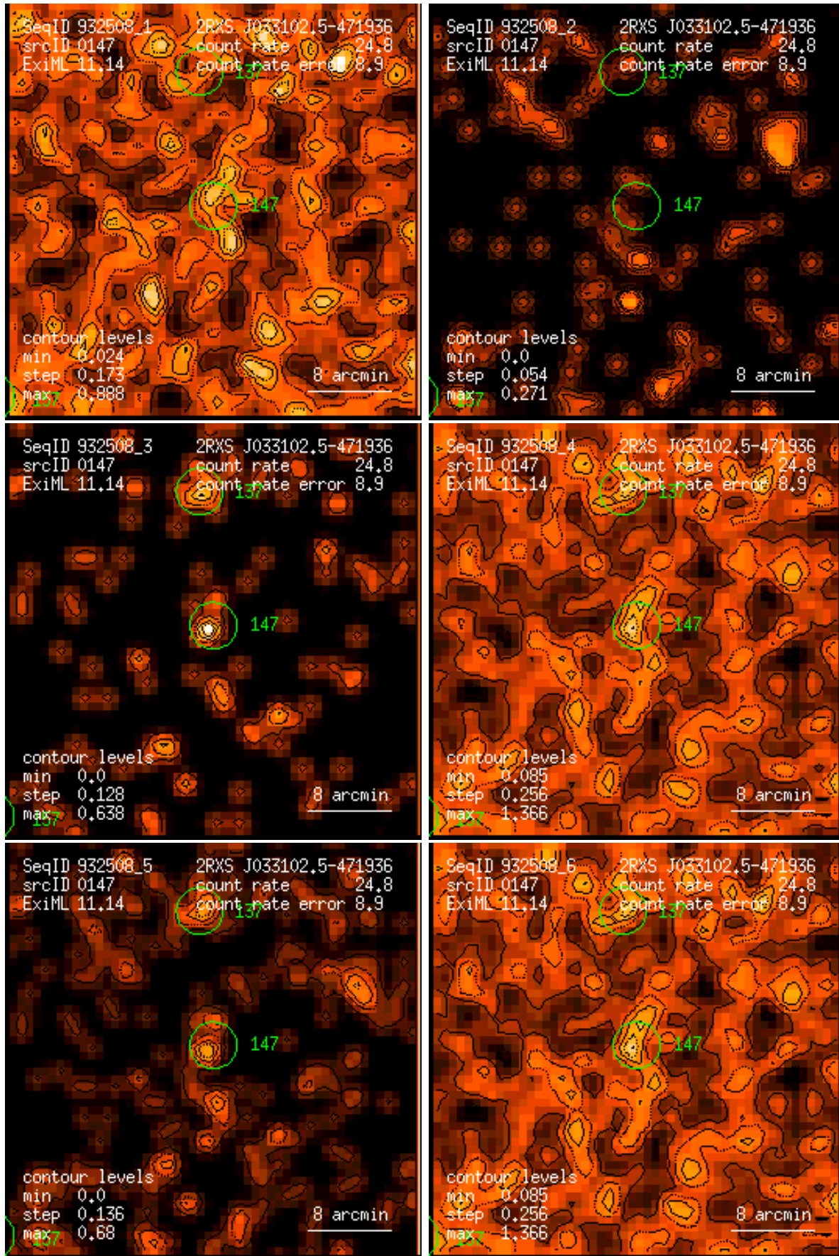
Figure 147: RASS 932508: detection 0147: band rate images, Gaussian filter: (1) PSPC channels 11 – 41, (2) 52 – 90, (3) 91 – 201, (4) 11 – 235, (5) 52 – 201, (6) 11 – 201. Broad band rates in counts/ks. Band rate contour levels in counts/ks/arcmin 2 .
