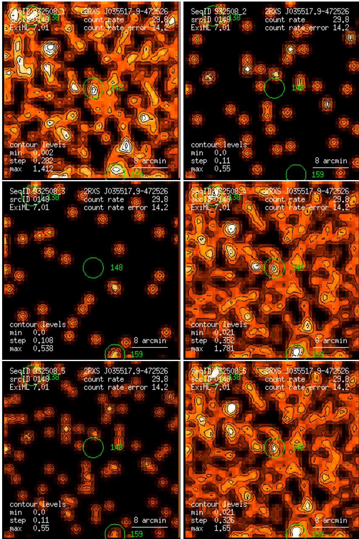
Figure 148: RASS 932508: detection 0148: band rate images, Gaussian filter: (1) PSPC channels 11 – 41, (2) 52 – 90, (3) 91 – 201, (4) 11 – 235, (5) 52 – 201, (6) 11 – 201. Broad band rates in counts/ks. Band rate contour levels in counts/ks/arcmin 2 .
