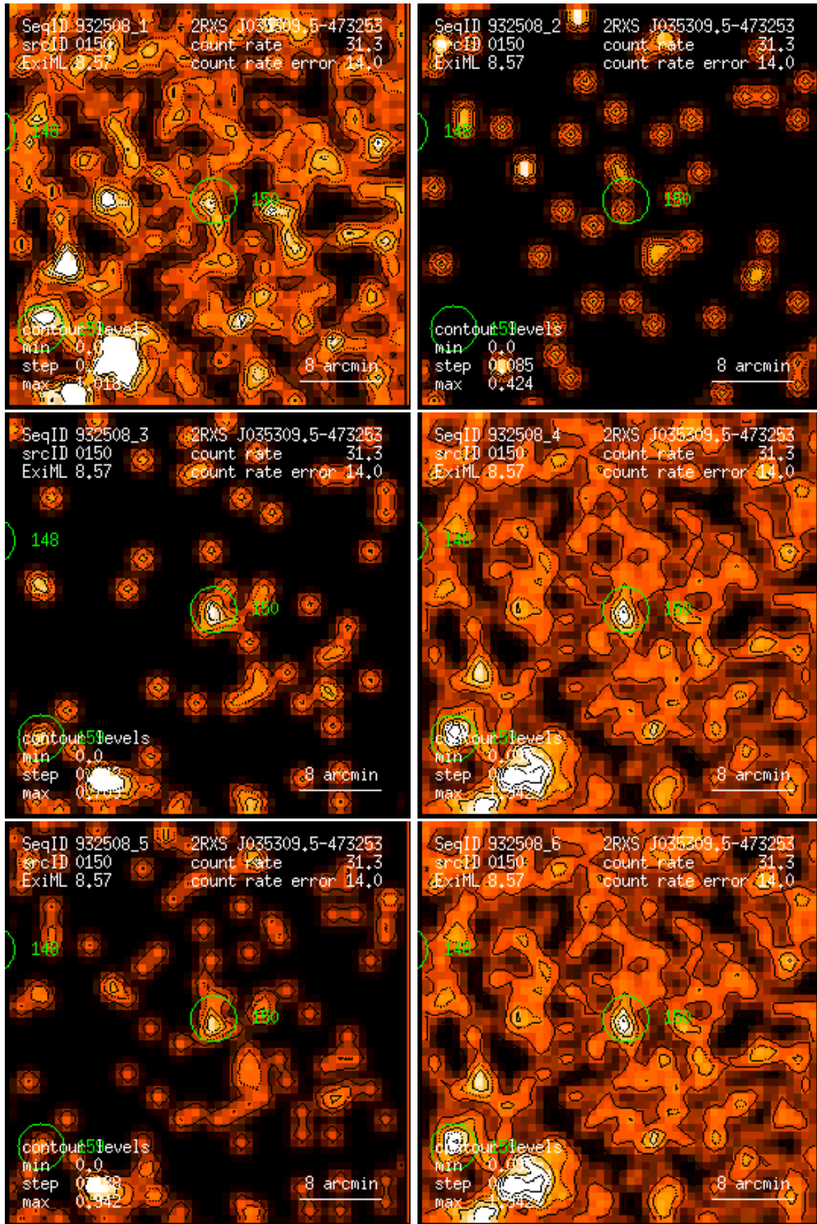
Figure 150: RASS 932508: detection 0150: band rate images, Gaussian filter: (1) PSPC channels 11 – 41, (2) 52 – 90, (3) 91 – 201, (4) 11 – 235, (5) 52 – 201, (6) 11 – 201. Broad band rates in counts/ks. Band rate contour levels in counts/ks/arcmin 2 .
