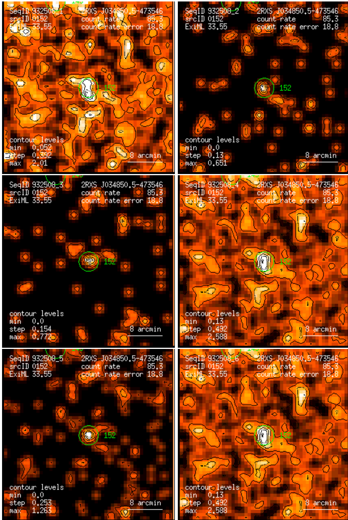
Figure 152: RASS 932508: detection 0152: band rate images, Gaussian filter: (1) PSPC channels 11 – 41, (2) 52 – 90, (3) 91 – 201, (4) 11 – 235, (5) 52 – 201, (6) 11 – 201. Broad band rates in counts/ks. Band rate contour levels in counts/ks/arcmin 2 .
