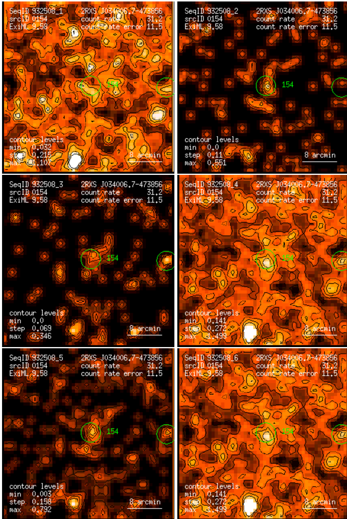
Figure 154: RASS 932508: detection 0154: band rate images, Gaussian filter: (1) PSPC channels 11 – 41, (2) 52 – 90, (3) 91 – 201, (4) 11 – 235, (5) 52 – 201, (6) 11 – 201. Broad band rates in counts/ks. Band rate contour levels in counts/ks/arcmin 2 .
