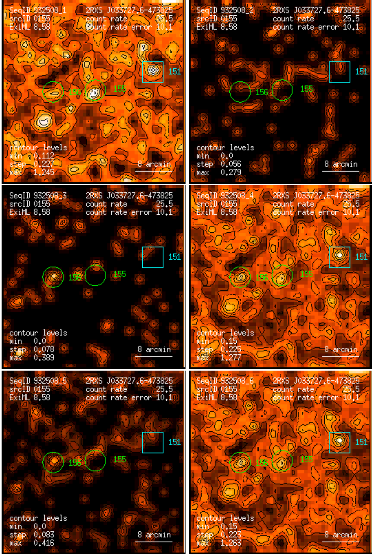
Figure 155: RASS 932508: detection 0155: band rate images, Gaussian filter: (1) PSPC channels 11 – 41, (2) 52 – 90, (3) 91 – 201, (4) 11 – 235, (5) 52 – 201, (6) 11 – 201. Broad band rates in counts/ks. Band rate contour levels in counts/ks/arcmin 2 .
