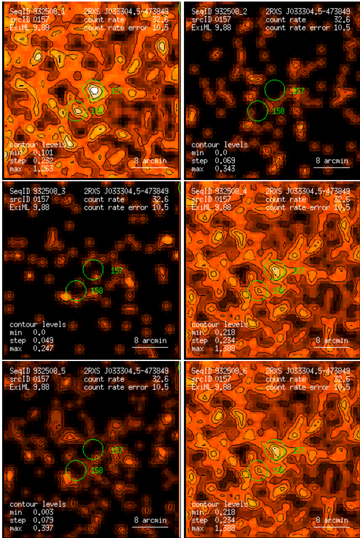
Figure 157: RASS 932508: detection 0157: band rate images, Gaussian filter: (1) PSPC channels 11 – 41, (2) 52 – 90, (3) 91 – 201, (4) 11 – 235, (5) 52 – 201, (6) 11 – 201. Broad band rates in counts/ks. Band rate contour levels in counts/ks/arcmin 2 .
