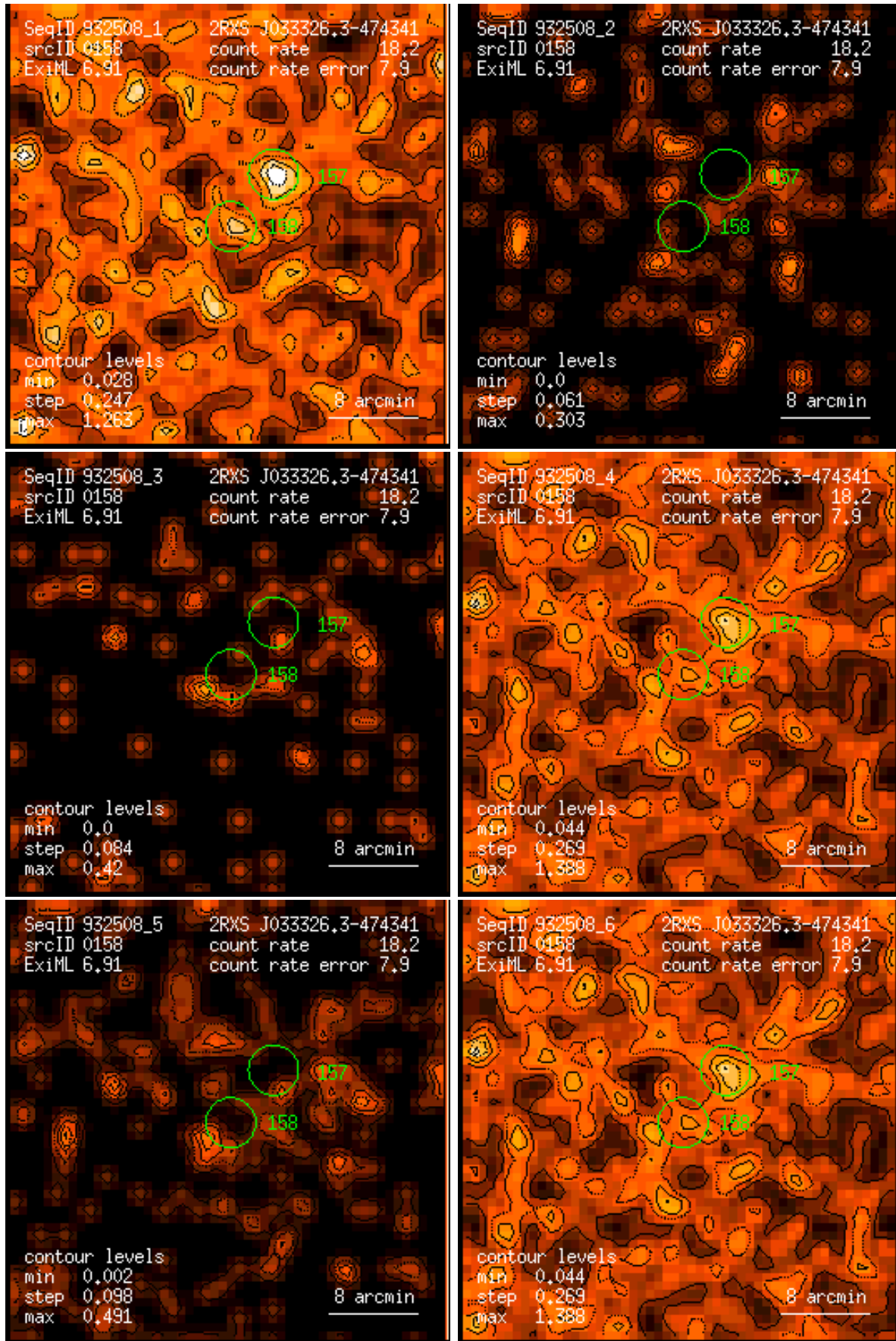
Figure 158: RASS 932508: detection 0158: band rate images, Gaussian filter: (1) PSPC channels 11 – 41, (2) 52 – 90, (3) 91 – 201, (4) 11 – 235, (5) 52 – 201, (6) 11 – 201. Broad band rates in counts/ks. Band rate contour levels in counts/ks/arcmin 2 .
